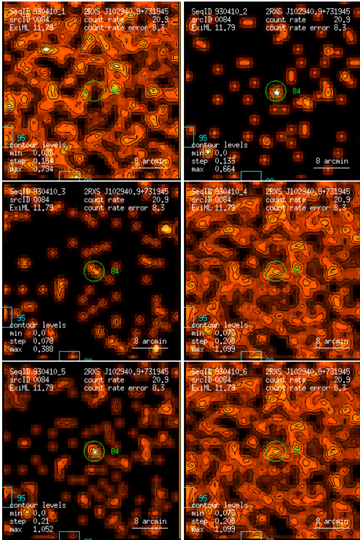
Figure 84: RASS 930410: detection 0084: band rate images, Gaussian filter: (1) PSPC channels 11 – 41, (2) 52 – 90, (3) 91 – 201, (4) 11 – 235, (5) 52 – 201, (6) 11 – 201. Broad band rates in counts/ks. Band rate contour levels in counts/ks/arcmin 2 .
