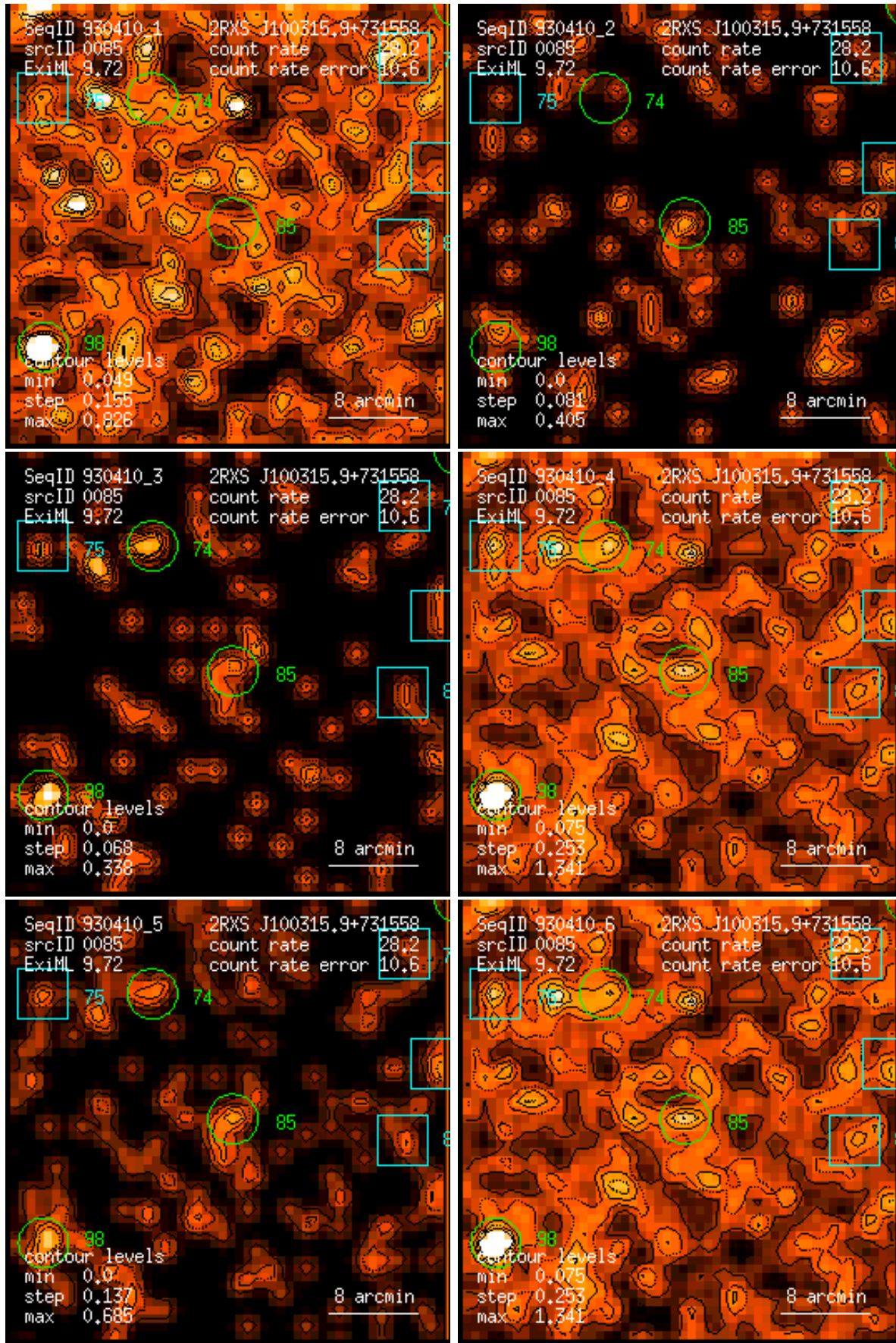
Figure 85: RASS 930410: detection 0085: band rate images, Gaussian filter: (1) PSPC channels 11 – 41, (2) 52 – 90, (3) 91 – 201, (4) 11 – 235, (5) 52 – 201, (6) 11 – 201. Broad band rates in counts/ks. Band rate contour levels in counts/ks/arcmin 2 .
