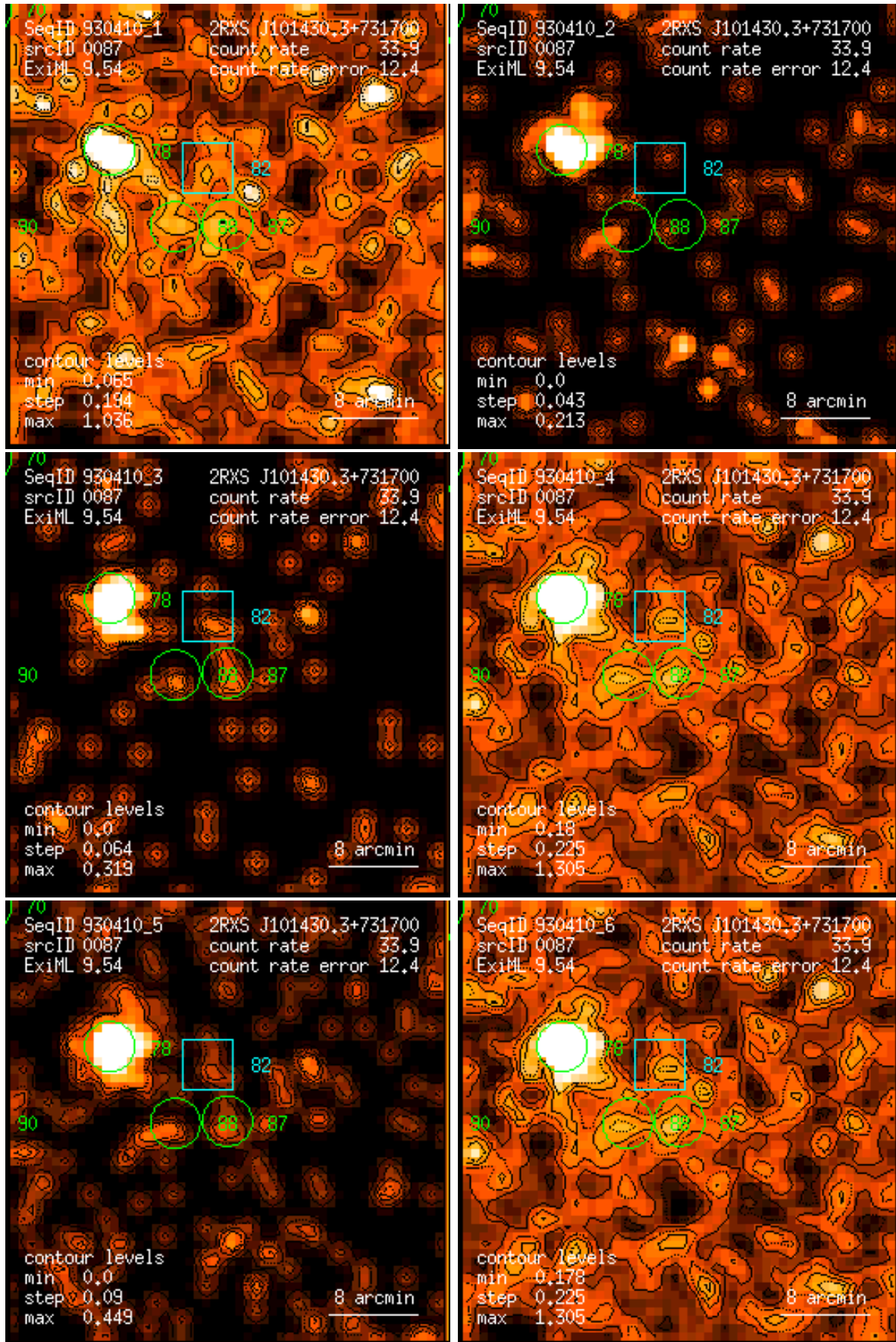
Figure 87: RASS 930410: detection 0087: band rate images, Gaussian filter: (1) PSPC channels 11 – 41, (2) 52 – 90, (3) 91 – 201, (4) 11 – 235, (5) 52 – 201, (6) 11 – 201. Broad band rates in counts/ks. Band rate contour levels in counts/ks/arcmin 2 .
