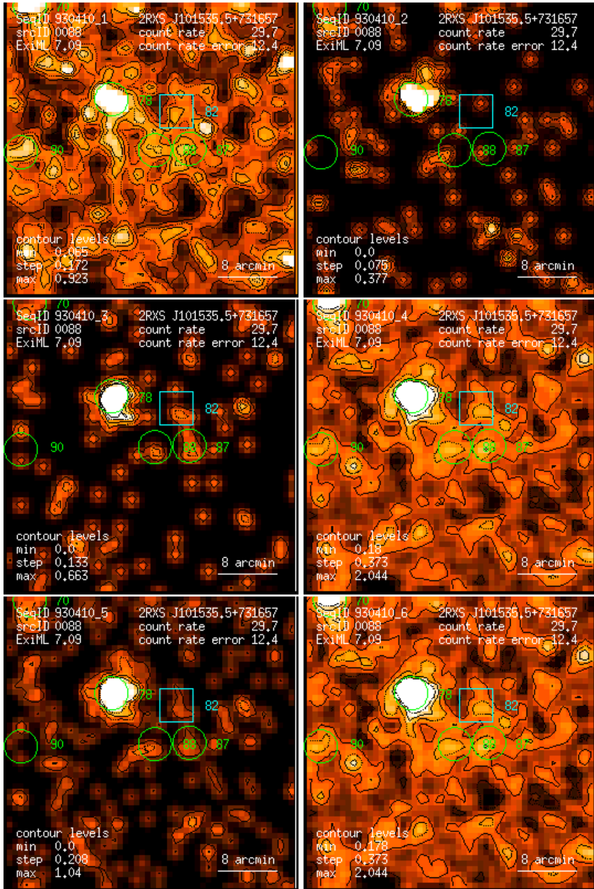
Figure 88: RASS 930410: detection 0088: band rate images, Gaussian filter: (1) PSPC channels 11 – 41, (2) 52 – 90, (3) 91 – 201, (4) 11 – 235, (5) 52 – 201, (6) 11 – 201. Broad band rates in counts/ks. Band rate contour levels in counts/ks/arcmin 2 .
