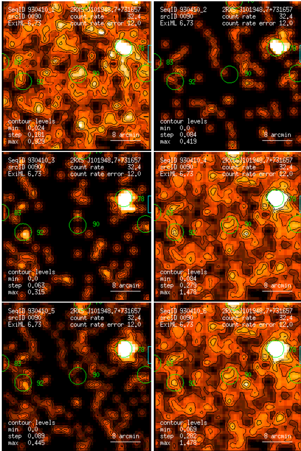
Figure 90: RASS 930410: detection 0090: band rate images, Gaussian filter: (1) PSPC channels 11 – 41, (2) 52 – 90, (3) 91 – 201, (4) 11 – 235, (5) 52 – 201, (6) 11 – 201. Broad band rates in counts/ks. Band rate contour levels in counts/ks/arcmin 2 .
