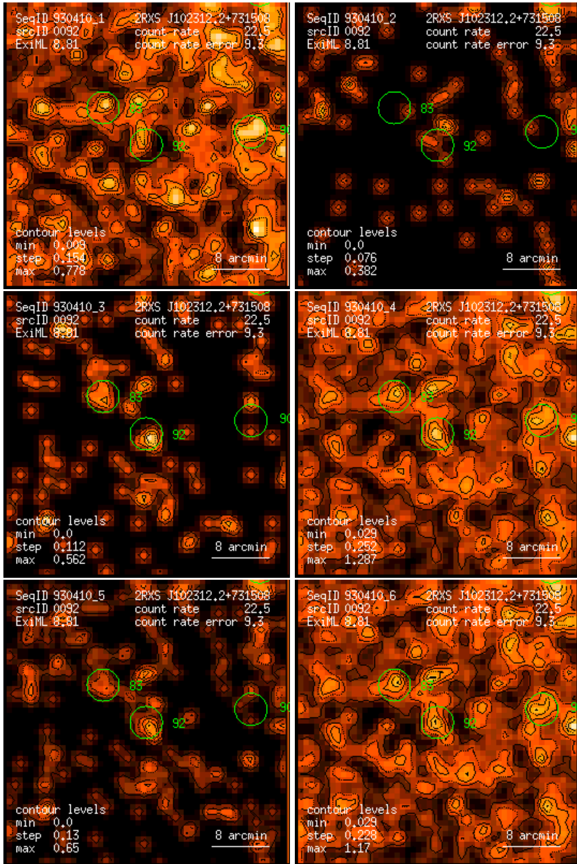
Figure 92: RASS 930410: detection 0092: band rate images, Gaussian filter: (1) PSPC channels 11 – 41, (2) 52 – 90, (3) 91 – 201, (4) 11 – 235, (5) 52 – 201, (6) 11 – 201. Broad band rates in counts/ks. Band rate contour levels in counts/ks/arcmin 2 .
