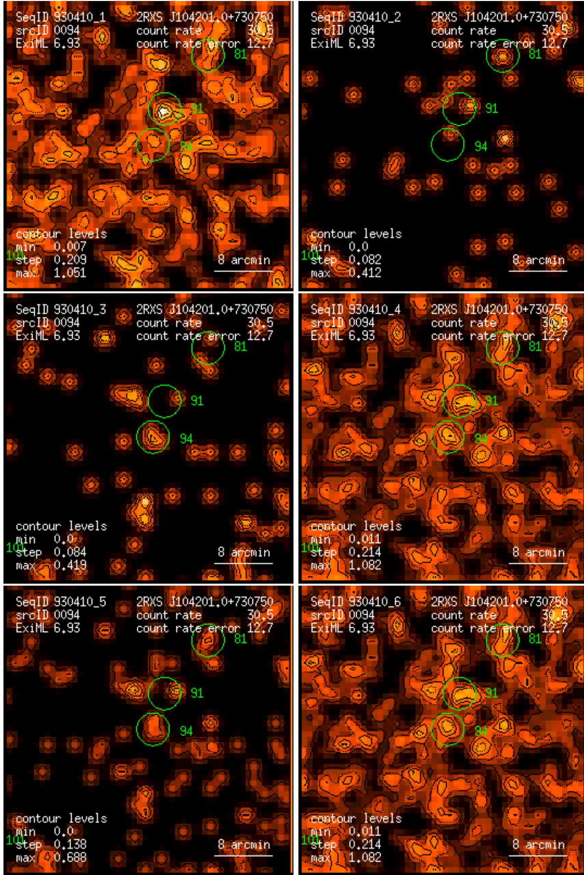
Figure 94: RASS 930410: detection 0094: band rate images, Gaussian filter: (1) PSPC channels 11 – 41, (2) 52 – 90, (3) 91 – 201, (4) 11 – 235, (5) 52 – 201, (6) 11 – 201. Broad band rates in counts/ks. Band rate contour levels in counts/ks/arcmin 2 .
