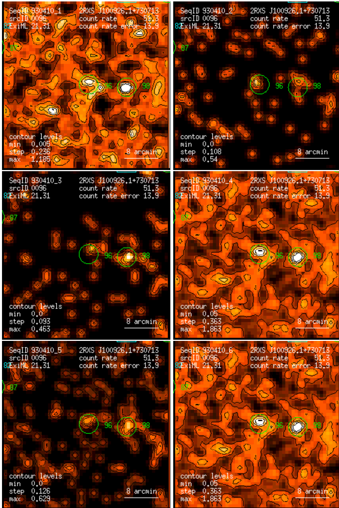
Figure 96: RASS 930410: detection 0096: band rate images, Gaussian filter: (1) PSPC channels 11 – 41, (2) 52 – 90, (3) 91 – 201, (4) 11 – 235, (5) 52 – 201, (6) 11 – 201. Broad band rates in counts/ks. Band rate contour levels in counts/ks/arcmin 2 .
