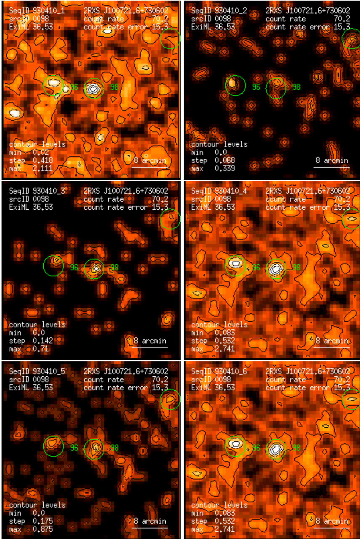
Figure 98: RASS 930410: detection 0098: band rate images, Gaussian filter: (1) PSPC channels 11 – 41, (2) 52 – 90, (3) 91 – 201, (4) 11 – 235, (5) 52 – 201, (6) 11 – 201. Broad band rates in counts/ks. Band rate contour levels in counts/ks/arcmin 2 .
