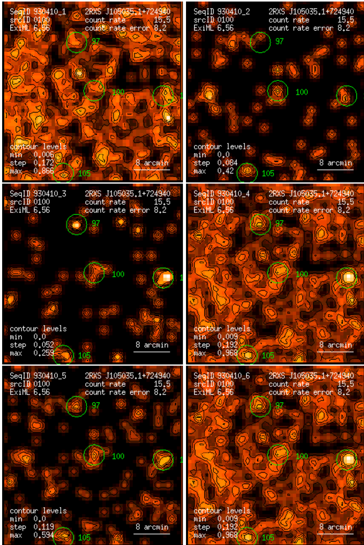
Figure 100: RASS 930410: detection 0100: band rate images, Gaussian filter: (1) PSPC channels 11 – 41, (2) 52 – 90, (3) 91 – 201, (4) 11 – 235, (5) 52 – 201, (6) 11 – 201. Broad band rates in counts/ks. Band rate contour levels in counts/ks/arcmin 2 .
