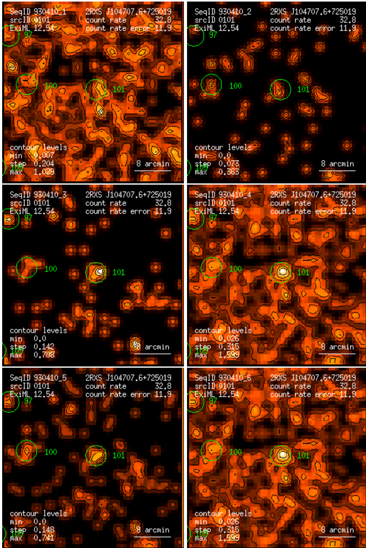
Figure 101: RASS 930410: detection 0101: band rate images, Gaussian filter: (1) PSPC channels 11 – 41, (2) 52 – 90, (3) 91 – 201, (4) 11 – 235, (5) 52 – 201, (6) 11 – 201. Broad band rates in counts/ks. Band rate contour levels in counts/ks/arcmin 2 .
