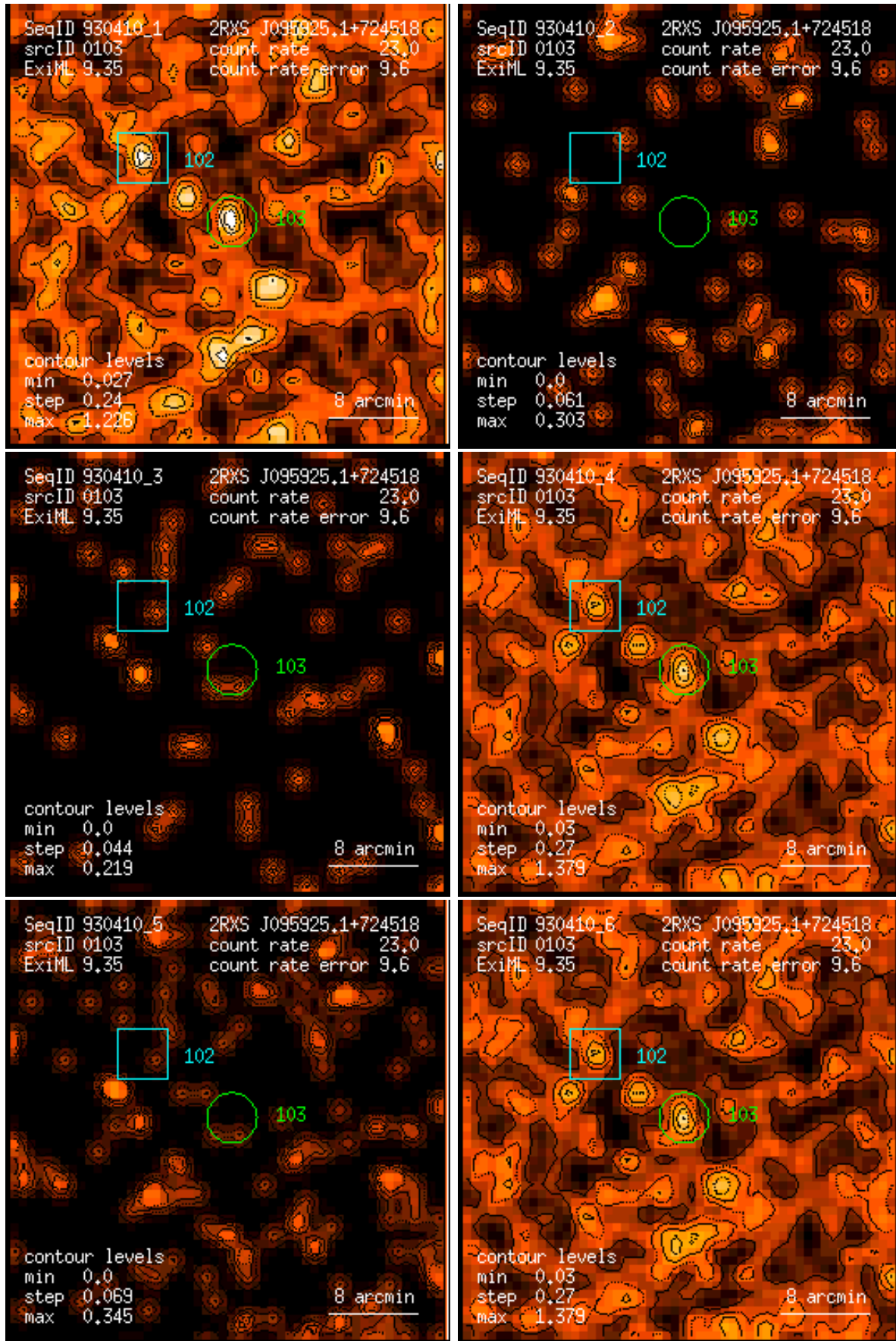
Figure 103: RASS 930410: detection 0103: band rate images, Gaussian filter: (1) PSPC channels 11 – 41, (2) 52 – 90, (3) 91 – 201, (4) 11 – 235, (5) 52 – 201, (6) 11 – 201. Broad band rates in counts/ks. Band rate contour levels in counts/ks/arcmin 2 .
