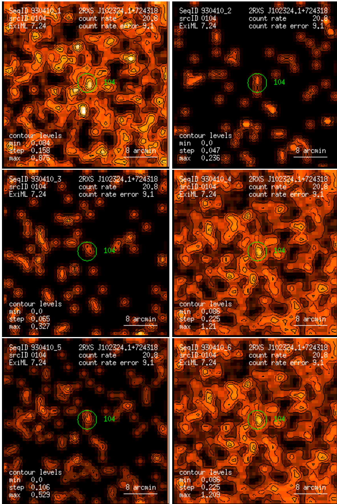
Figure 104: RASS 930410: detection 0104: band rate images, Gaussian filter: (1) PSPC channels 11 – 41, (2) 52 – 90, (3) 91 – 201, (4) 11 – 235, (5) 52 – 201, (6) 11 – 201. Broad band rates in counts/ks. Band rate contour levels in counts/ks/arcmin 2 .
