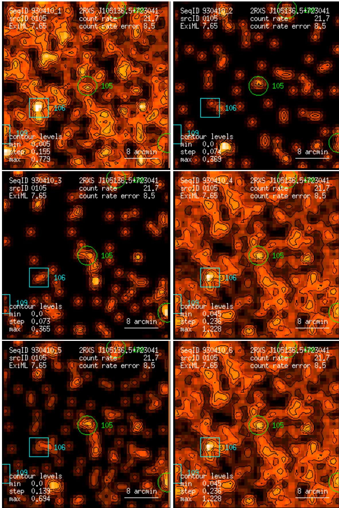
Figure 105: RASS 930410: detection 0105: band rate images, Gaussian filter: (1) PSPC channels 11 – 41, (2) 52 – 90, (3) 91 – 201, (4) 11 – 235, (5) 52 – 201, (6) 11 – 201. Broad band rates in counts/ks. Band rate contour levels in counts/ks/arcmin 2 .
