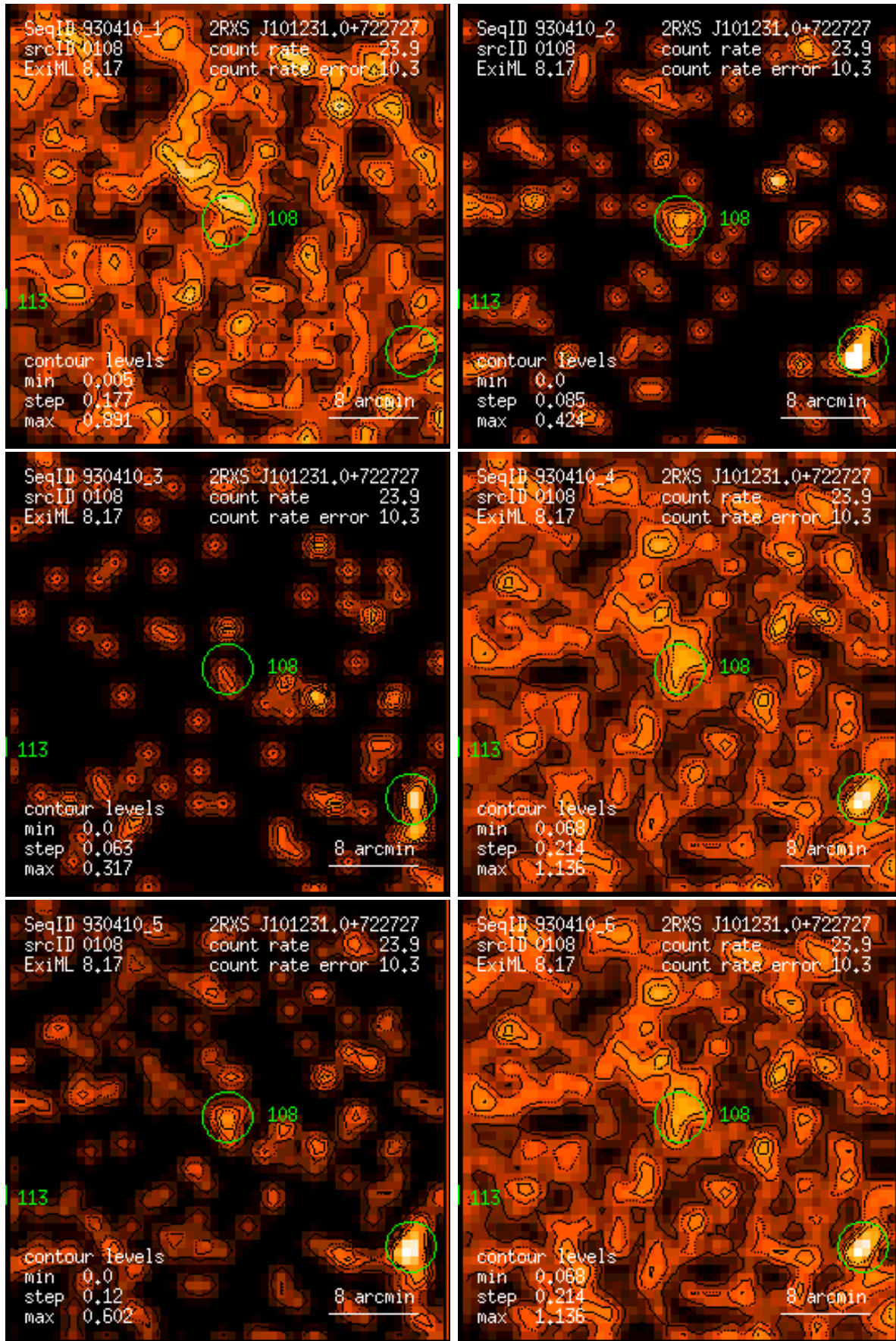
Figure 108: RASS 930410: detection 0108: band rate images, Gaussian filter: (1) PSPC channels 11 – 41, (2) 52 – 90, (3) 91 – 201, (4) 11 – 235, (5) 52 – 201, (6) 11 – 201. Broad band rates in counts/ks. Band rate contour levels in counts/ks/arcmin 2 .
