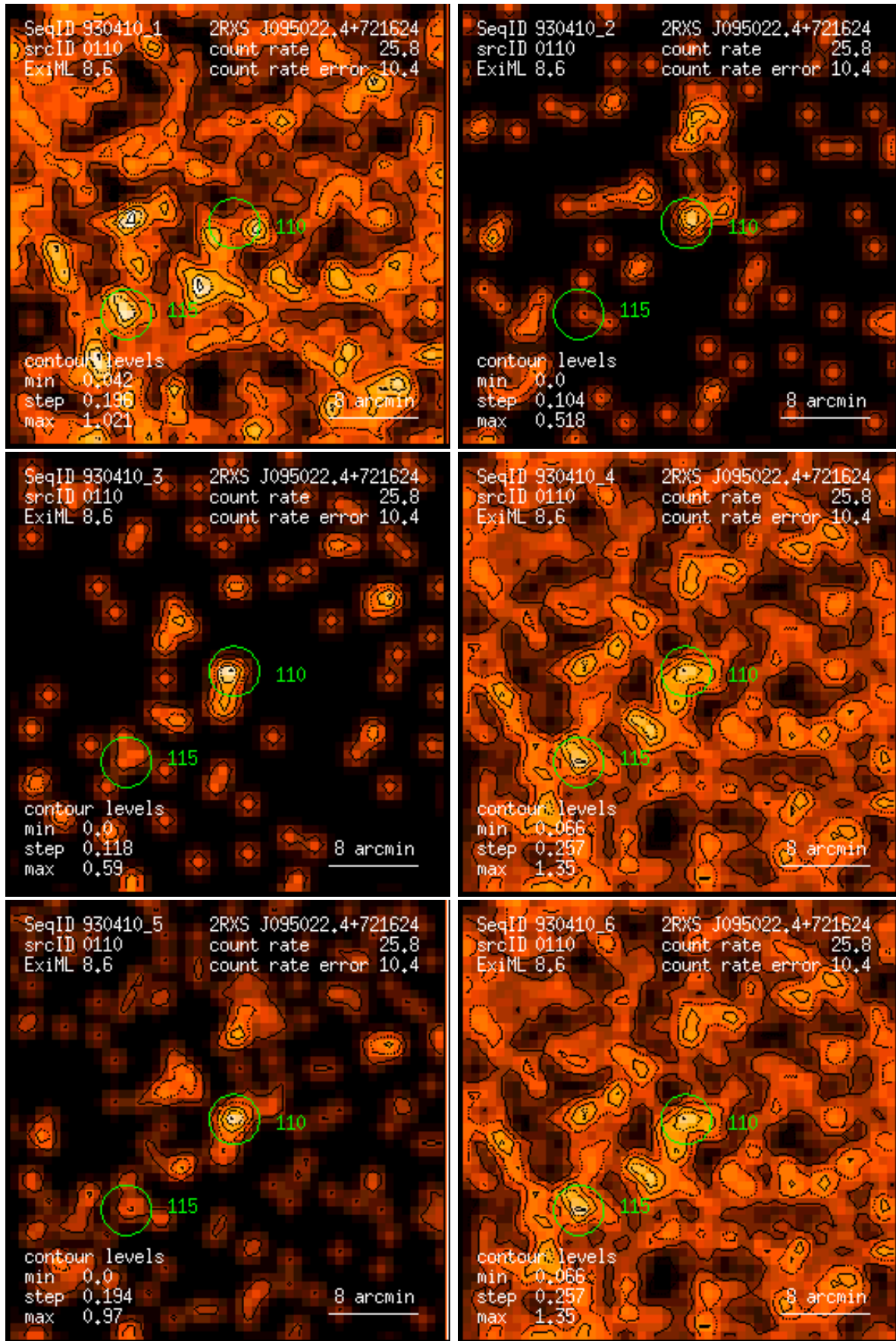
Figure 110: RASS 930410: detection 0110: band rate images, Gaussian filter: (1) PSPC channels 11 – 41, (2) 52 – 90, (3) 91 – 201, (4) 11 – 235, (5) 52 – 201, (6) 11 – 201. Broad band rates in counts/ks. Band rate contour levels in counts/ks/arcmin 2 .
