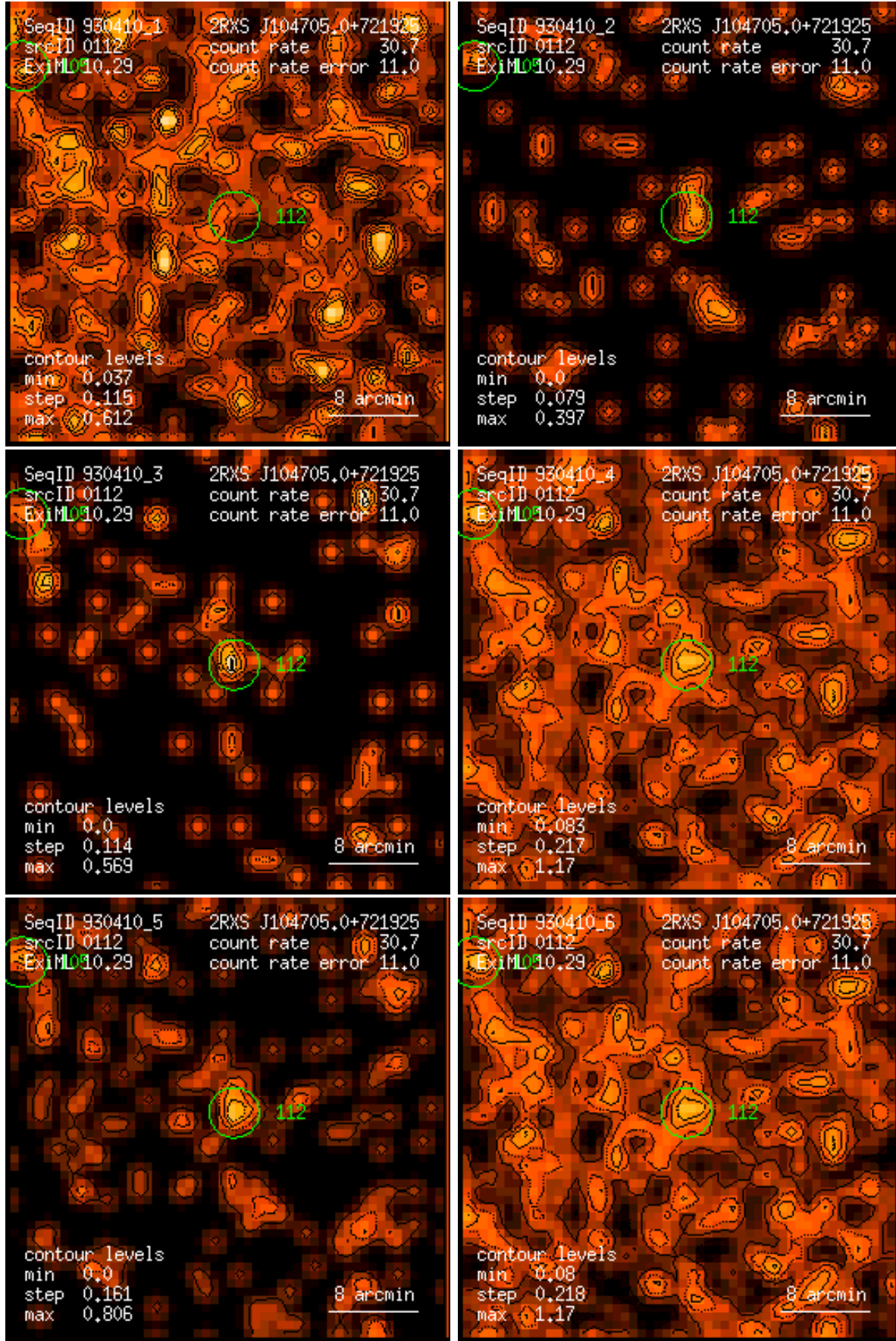
Figure 112: RASS 930410: detection 0112: band rate images, Gaussian filter: (1) PSPC channels 11 – 41, (2) 52 – 90, (3) 91 – 201, (4) 11 – 235, (5) 52 – 201, (6) 11 – 201. Broad band rates in counts/ks. Band rate contour levels in counts/ks/arcmin 2 .
