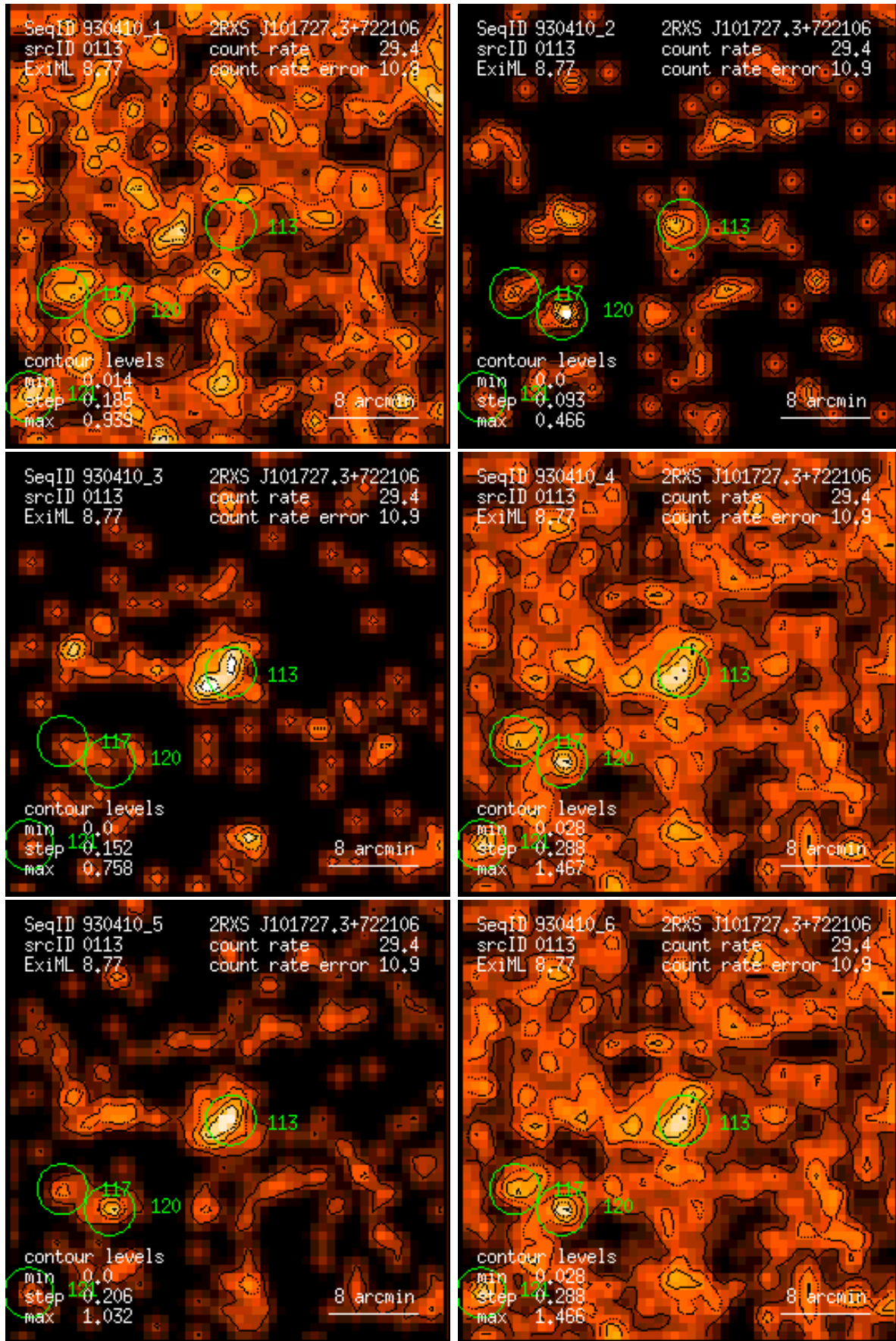
Figure 113: RASS 930410: detection 0113: band rate images, Gaussian filter: (1) PSPC channels 11 – 41, (2) 52 – 90, (3) 91 – 201, (4) 11 – 235, (5) 52 – 201, (6) 11 – 201. Broad band rates in counts/ks. Band rate contour levels in counts/ks/arcmin 2 .
