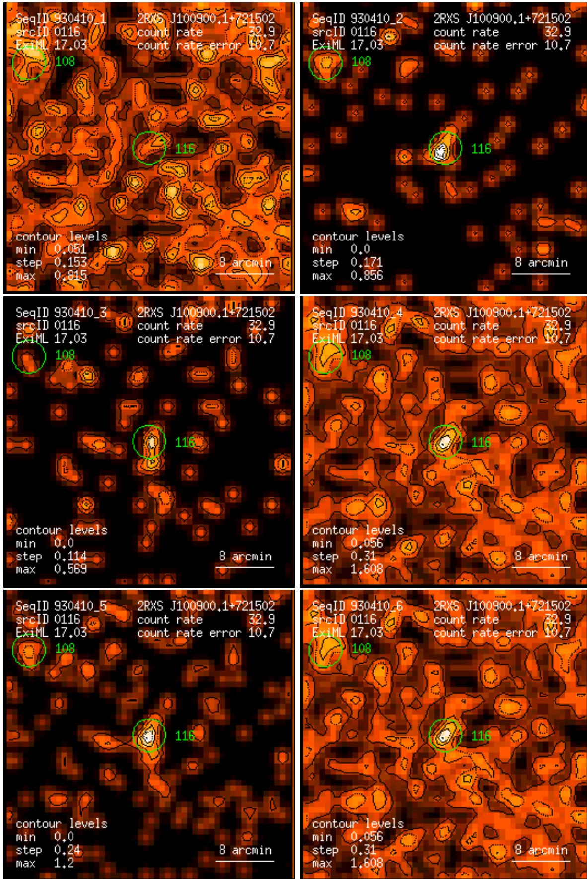
Figure 116: RASS 930410: detection 0116: band rate images, Gaussian filter: (1) PSPC channels 11 – 41, (2) 52 – 90, (3) 91 – 201, (4) 11 – 235, (5) 52 – 201, (6) 11 – 201. Broad band rates in counts/ks. Band rate contour levels in counts/ks/arcmin 2 .
