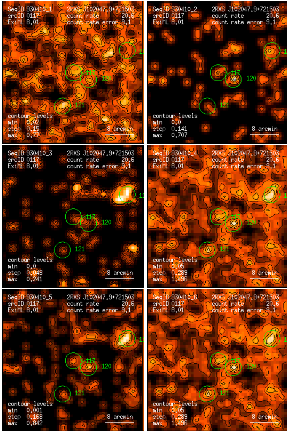
Figure 117: RASS 930410: detection 0117: band rate images, Gaussian filter: (1) PSPC channels 11 – 41, (2) 52 – 90, (3) 91 – 201, (4) 11 – 235, (5) 52 – 201, (6) 11 – 201. Broad band rates in counts/ks. Band rate contour levels in counts/ks/arcmin 2 .
