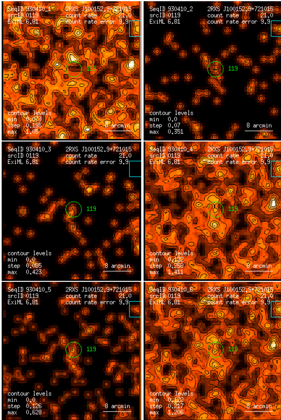
Figure 119: RASS 930410: detection 0119: band rate images, Gaussian filter: (1) PSPC channels 11 – 41, (2) 52 – 90, (3) 91 – 201, (4) 11 – 235, (5) 52 – 201, (6) 11 – 201. Broad band rates in counts/ks. Band rate contour levels in counts/ks/arcmin 2 .
