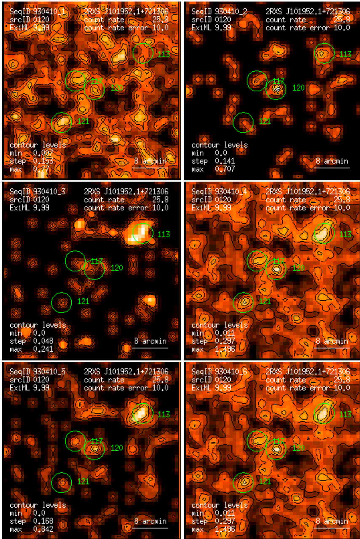
Figure 120: RASS 930410: detection 0120: band rate images, Gaussian filter: (1) PSPC channels 11 – 41, (2) 52 – 90, (3) 91 – 201, (4) 11 – 235, (5) 52 – 201, (6) 11 – 201. Broad band rates in counts/ks. Band rate contour levels in counts/ks/arcmin 2 .
