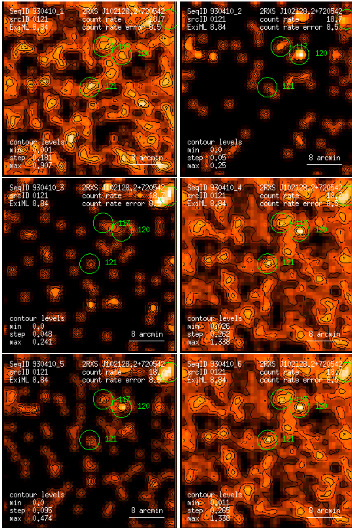
Figure 121: RASS 930410: detection 0121: band rate images, Gaussian filter: (1) PSPC channels 11 – 41, (2) 52 – 90, (3) 91 – 201, (4) 11 – 235, (5) 52 – 201, (6) 11 – 201. Broad band rates in counts/ks. Band rate contour levels in counts/ks/arcmin 2 .
