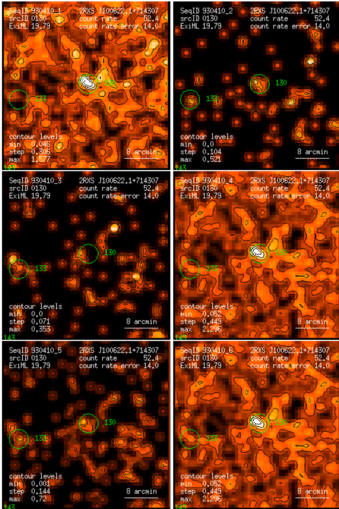
Figure 130: RASS 930410: detection 0130: band rate images, Gaussian filter: (1) PSPC channels 11 – 41, (2) 52 – 90, (3) 91 – 201, (4) 11 – 235, (5) 52 – 201, (6) 11 – 201. Broad band rates in counts/ks. Band rate contour levels in counts/ks/arcmin 2 .
