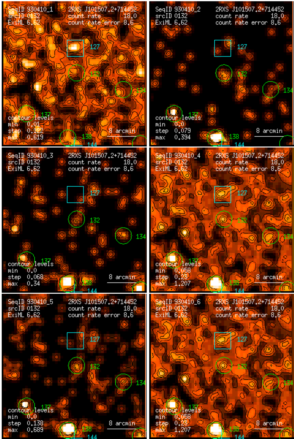
Figure 132: RASS 930410: detection 0132: band rate images, Gaussian filter: (1) PSPC channels 11 – 41, (2) 52 – 90, (3) 91 – 201, (4) 11 – 235, (5) 52 – 201, (6) 11 – 201. Broad band rates in counts/ks. Band rate contour levels in counts/ks/arcmin 2 .
