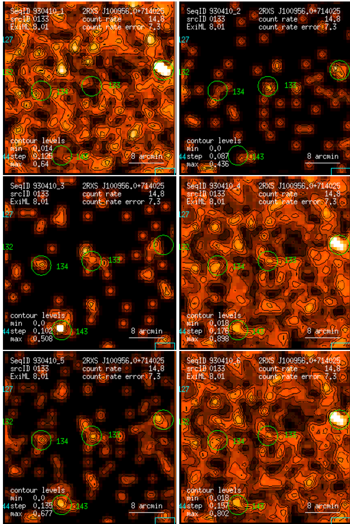
Figure 133: RASS 930410: detection 0133: band rate images, Gaussian filter: (1) PSPC channels 11 – 41, (2) 52 – 90, (3) 91 – 201, (4) 11 – 235, (5) 52 – 201, (6) 11 – 201. Broad band rates in counts/ks. Band rate contour levels in counts/ks/arcmin 2 .
