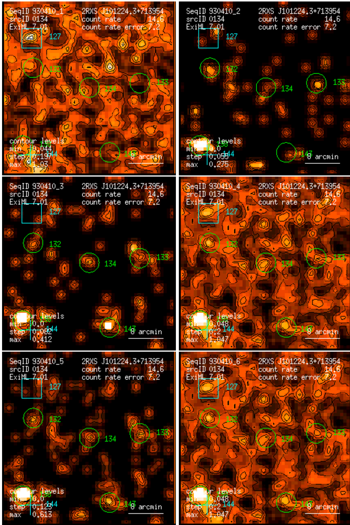
Figure 134: RASS 930410: detection 0134: band rate images, Gaussian filter: (1) PSPC channels 11 – 41, (2) 52 – 90, (3) 91 – 201, (4) 11 – 235, (5) 52 – 201, (6) 11 – 201. Broad band rates in counts/ks. Band rate contour levels in counts/ks/arcmin 2 .
