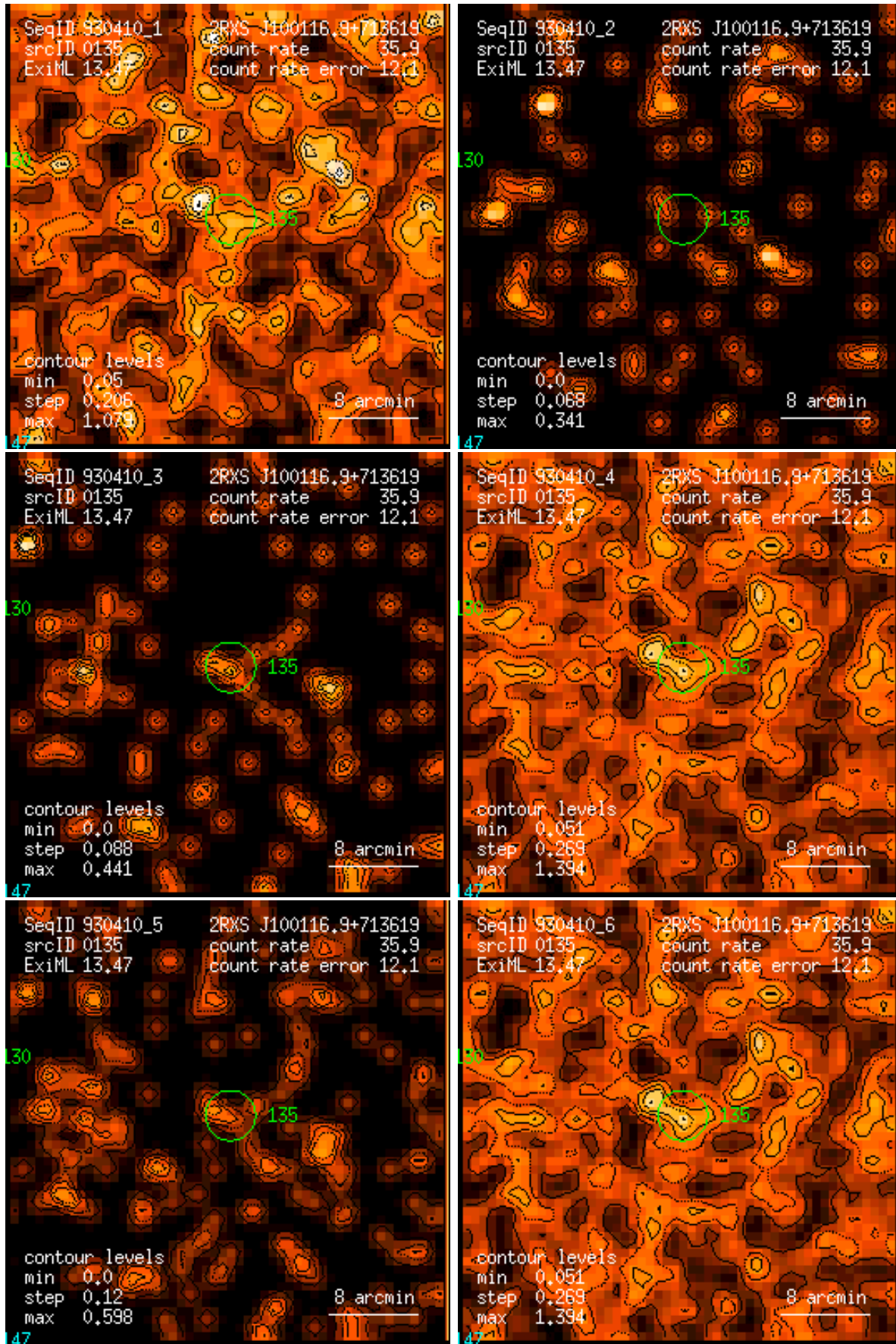
Figure 135: RASS 930410: detection 0135: band rate images, Gaussian filter: (1) PSPC channels 11 – 41, (2) 52 – 90, (3) 91 – 201, (4) 11 – 235, (5) 52 – 201, (6) 11 – 201. Broad band rates in counts/ks. Band rate contour levels in counts/ks/arcmin 2 .
