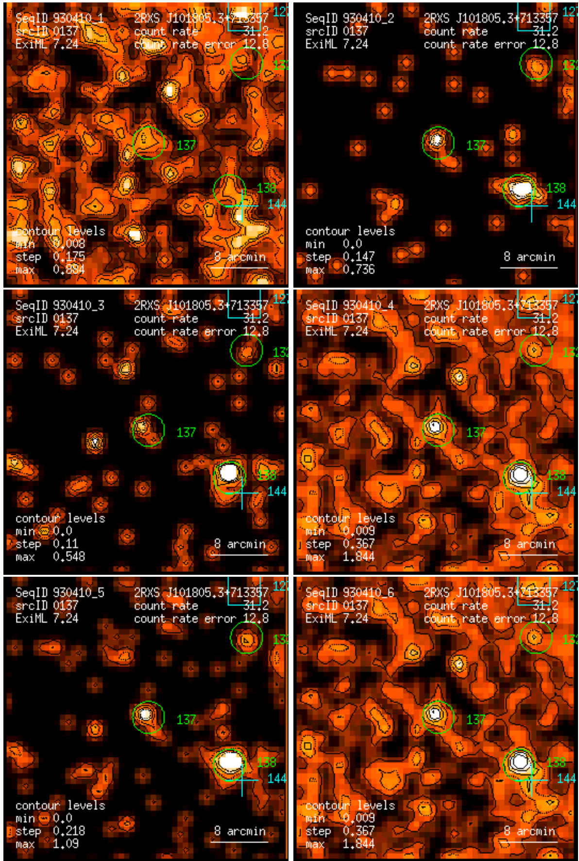
Figure 137: RASS 930410: detection 0137: band rate images, Gaussian filter: (1) PSPC channels 11 – 41, (2) 52 – 90, (3) 91 – 201, (4) 11 – 235, (5) 52 – 201, (6) 11 – 201. Broad band rates in counts/ks. Band rate contour levels in counts/ks/arcmin 2 .
