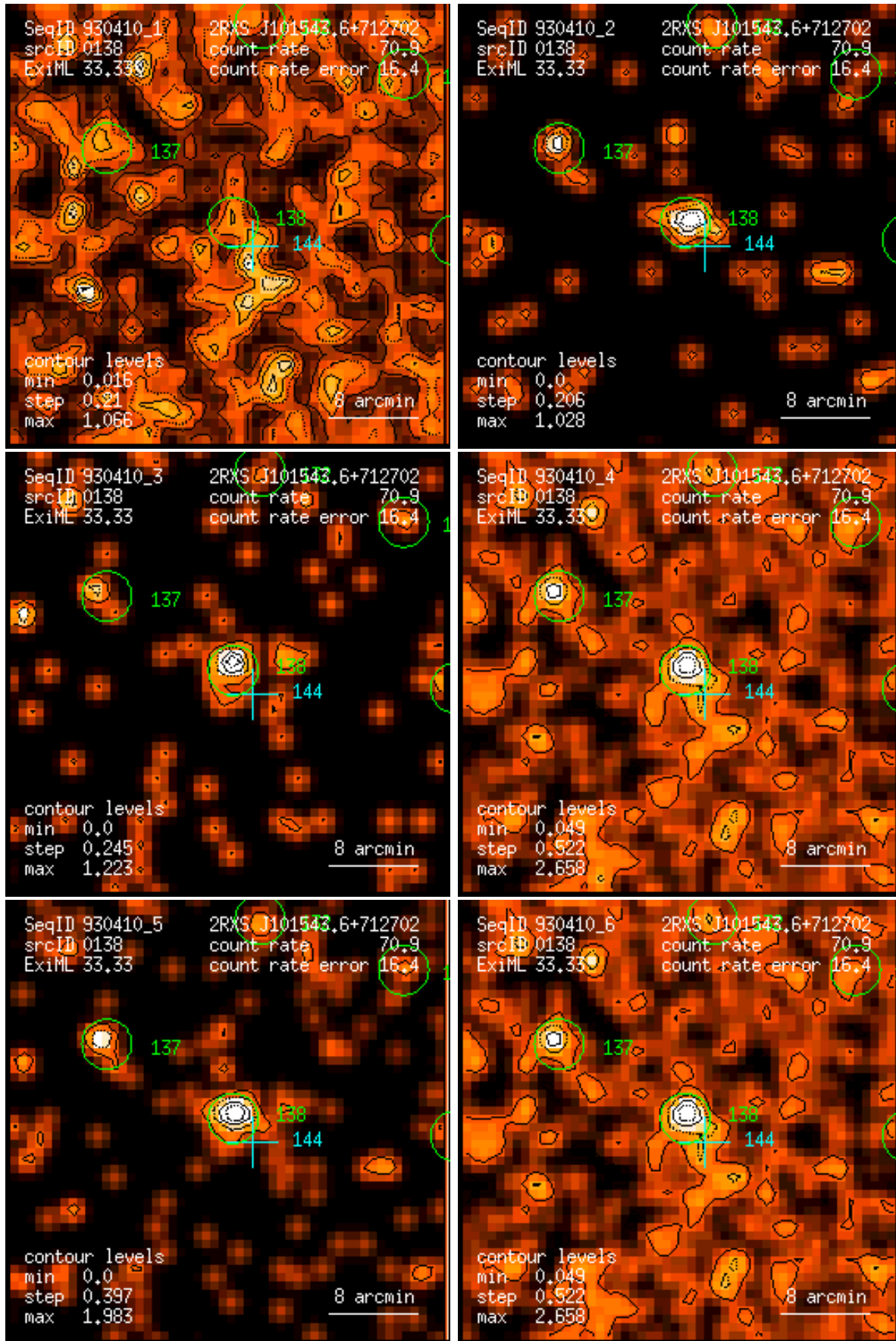
Figure 138: RASS 930410: detection 0138: band rate images, Gaussian filter: (1) PSPC channels 11 – 41, (2) 52 – 90, (3) 91 – 201, (4) 11 – 235, (5) 52 – 201, (6) 11 – 201. Broad band rates in counts/ks. Band rate contour levels in counts/ks/arcmin 2 .
