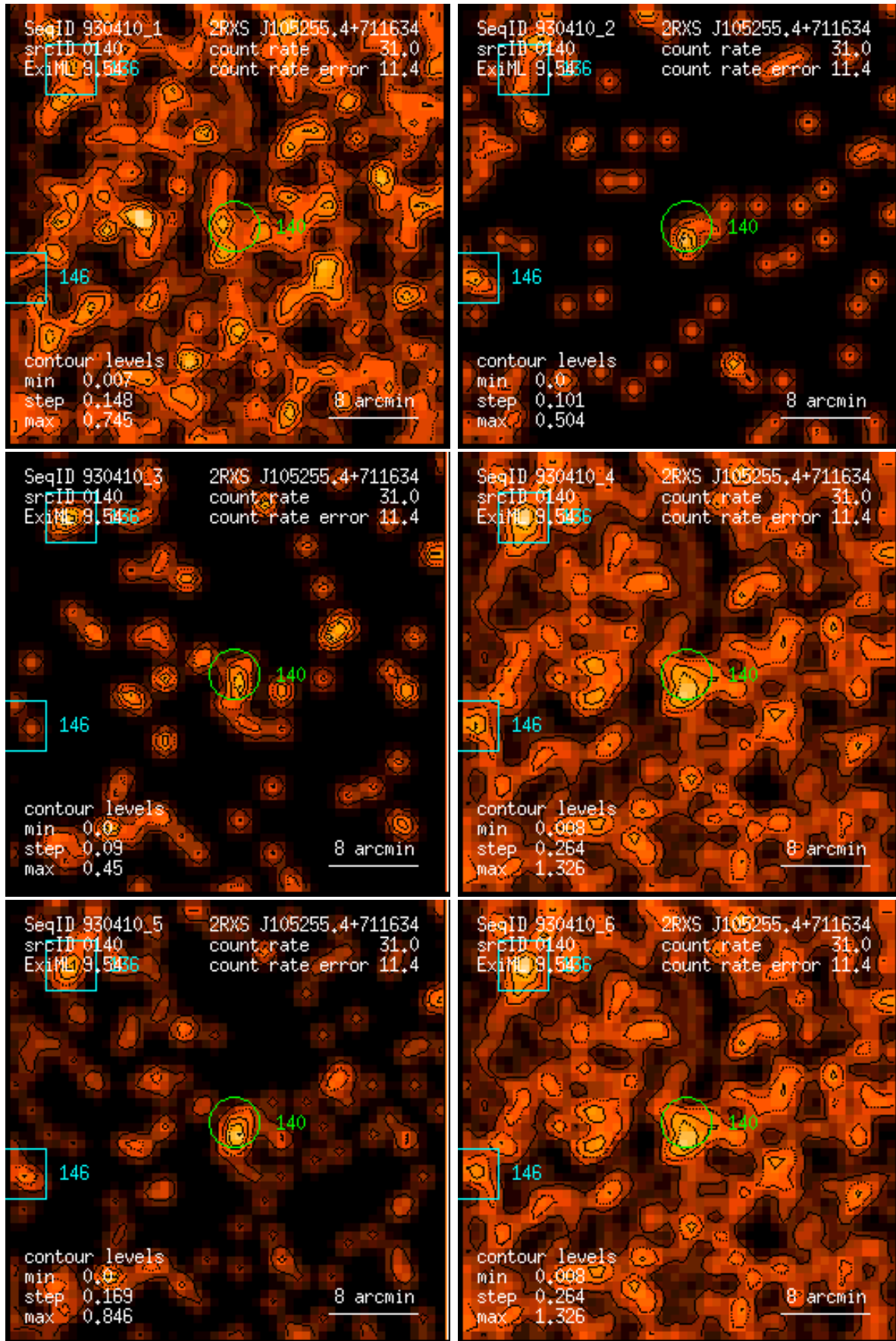
Figure 140: RASS 930410: detection 0140: band rate images, Gaussian filter: (1) PSPC channels 11 – 41, (2) 52 – 90, (3) 91 – 201, (4) 11 – 235, (5) 52 – 201, (6) 11 – 201. Broad band rates in counts/ks. Band rate contour levels in counts/ks/arcmin 2 .
