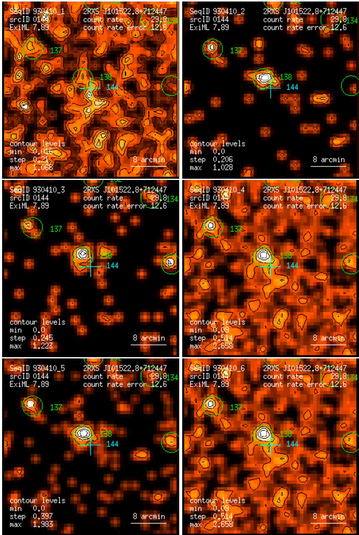
Figure 144: RASS 930410: detection 0144: band rate images, Gaussian filter: (1) PSPC channels 11 – 41, (2) 52 – 90, (3) 91 – 201, (4) 11 – 235, (5) 52 – 201, (6) 11 – 201. Broad band rates in counts/ks. Band rate contour levels in counts/ks/arcmin 2 .
