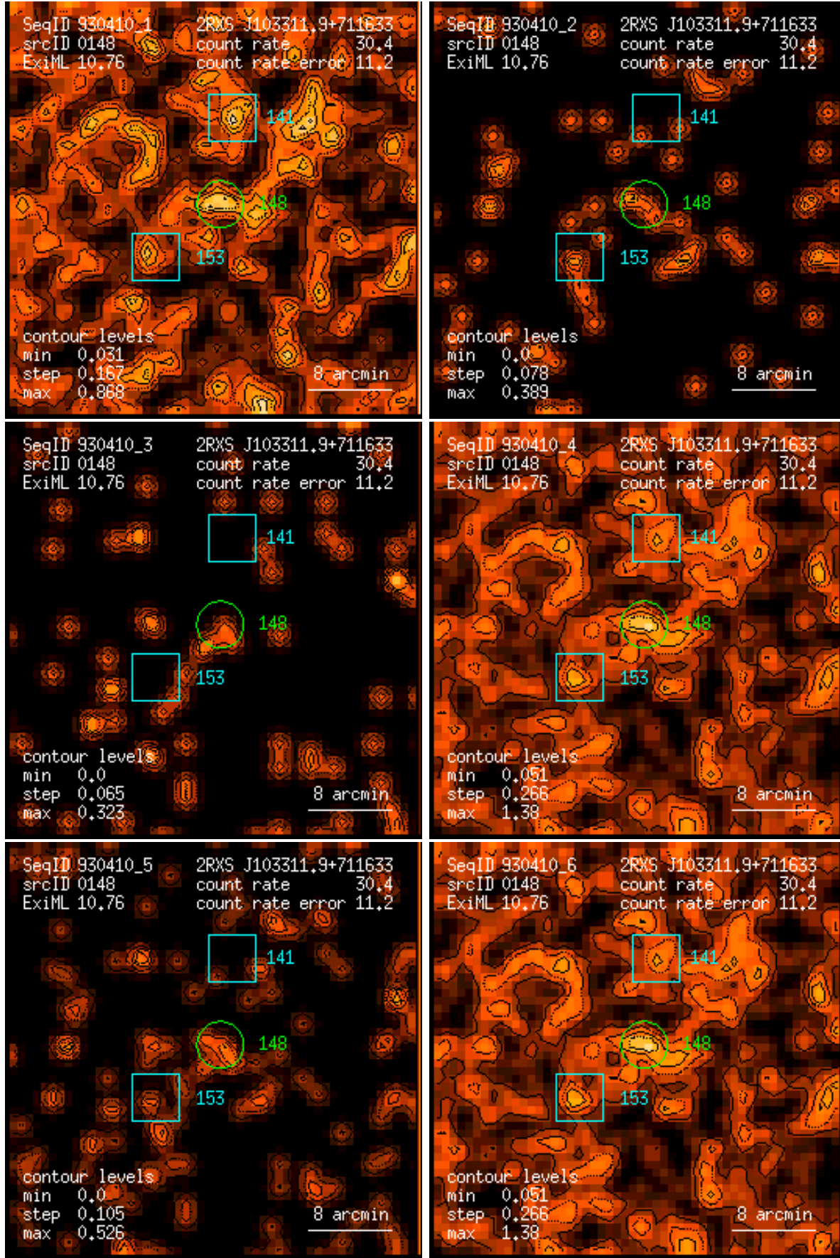
Figure 148: RASS 930410: detection 0148: band rate images, Gaussian filter: (1) PSPC channels 11 – 41, (2) 52 – 90, (3) 91 – 201, (4) 11 – 235, (5) 52 – 201, (6) 11 – 201. Broad band rates in counts/ks. Band rate contour levels in counts/ks/arcmin 2 .
