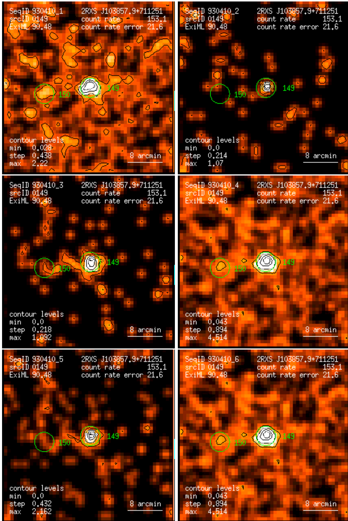
Figure 149: RASS 930410: detection 0149: band rate images, Gaussian filter: (1) PSPC channels 11 – 41, (2) 52 – 90, (3) 91 – 201, (4) 11 – 235, (5) 52 – 201, (6) 11 – 201. Broad band rates in counts/ks. Band rate contour levels in counts/ks/arcmin 2 .
