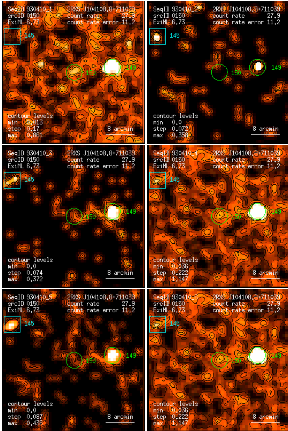
Figure 150: RASS 930410: detection 0150: band rate images, Gaussian filter: (1) PSPC channels 11 – 41, (2) 52 – 90, (3) 91 – 201, (4) 11 – 235, (5) 52 – 201, (6) 11 – 201. Broad band rates in counts/ks. Band rate contour levels in counts/ks/arcmin 2 .
