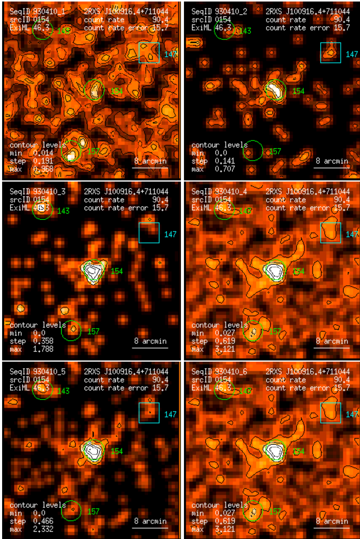
Figure 154: RASS 930410: detection 0154: band rate images, Gaussian filter: (1) PSPC channels 11 – 41, (2) 52 – 90, (3) 91 – 201, (4) 11 – 235, (5) 52 – 201, (6) 11 – 201. Broad band rates in counts/ks. Band rate contour levels in counts/ks/arcmin 2 .
