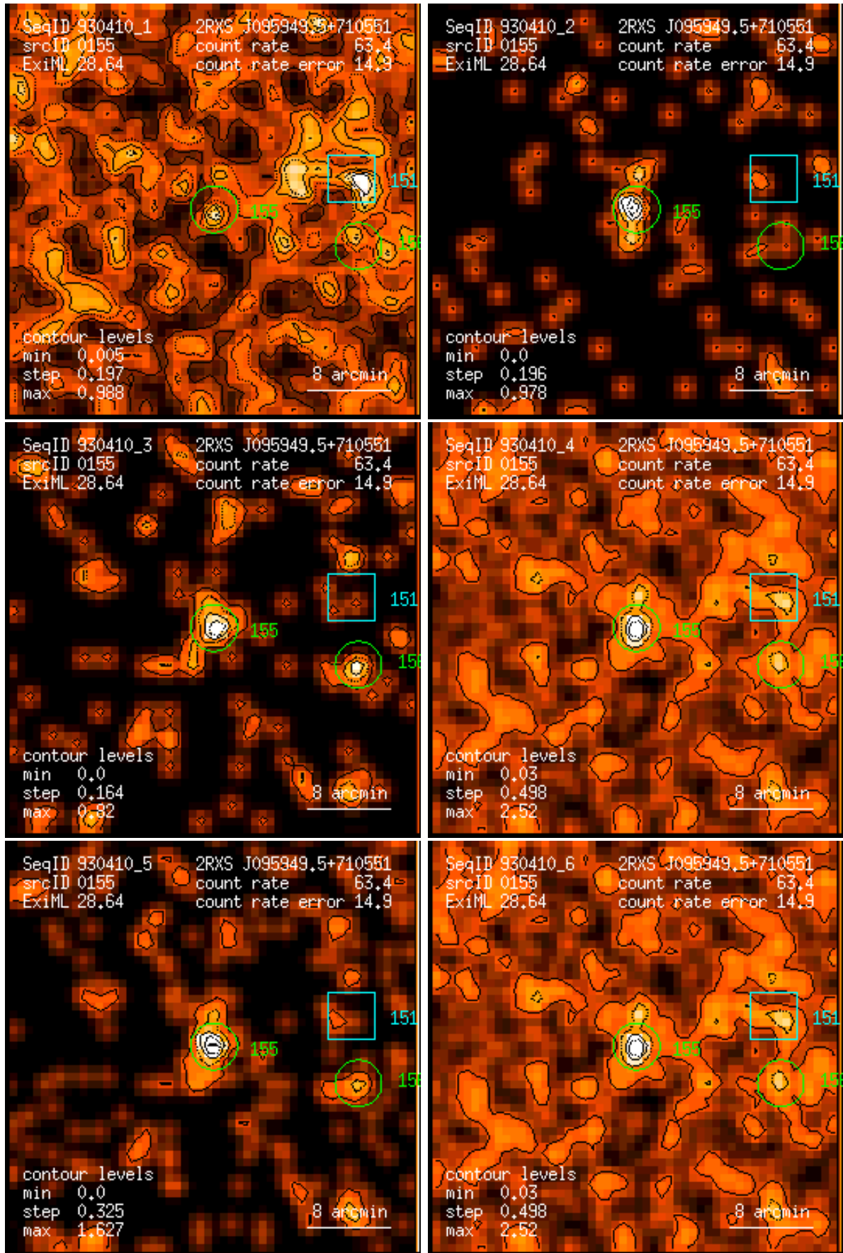
Figure 155: RASS 930410: detection 0155: band rate images, Gaussian filter: (1) PSPC channels 11 – 41, (2) 52 – 90, (3) 91 – 201, (4) 11 – 235, (5) 52 – 201, (6) 11 – 201. Broad band rates in counts/ks. Band rate contour levels in counts/ks/arcmin 2 .
