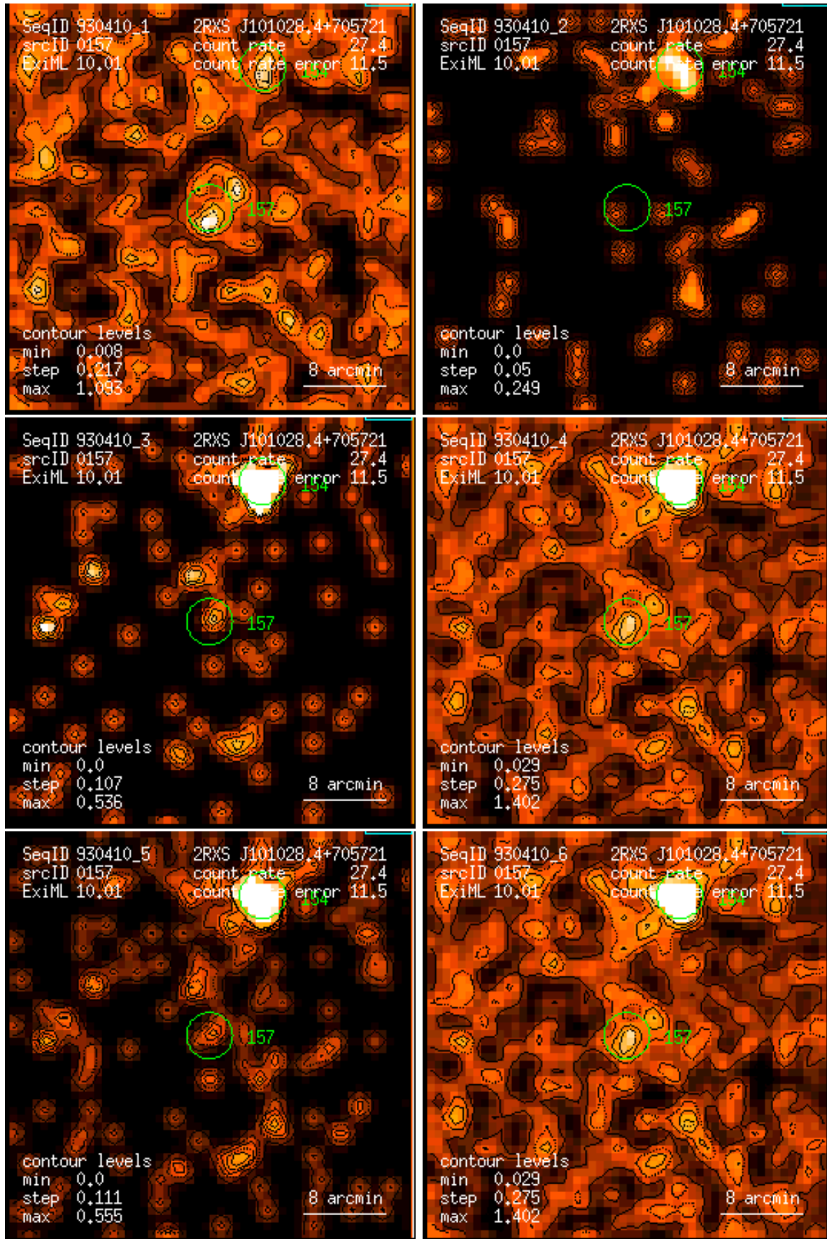
Figure 157: RASS 930410: detection 0157: band rate images, Gaussian filter: (1) PSPC channels 11 – 41, (2) 52 – 90, (3) 91 – 201, (4) 11 – 235, (5) 52 – 201, (6) 11 – 201. Broad band rates in counts/ks. Band rate contour levels in counts/ks/arcmin 2 .
