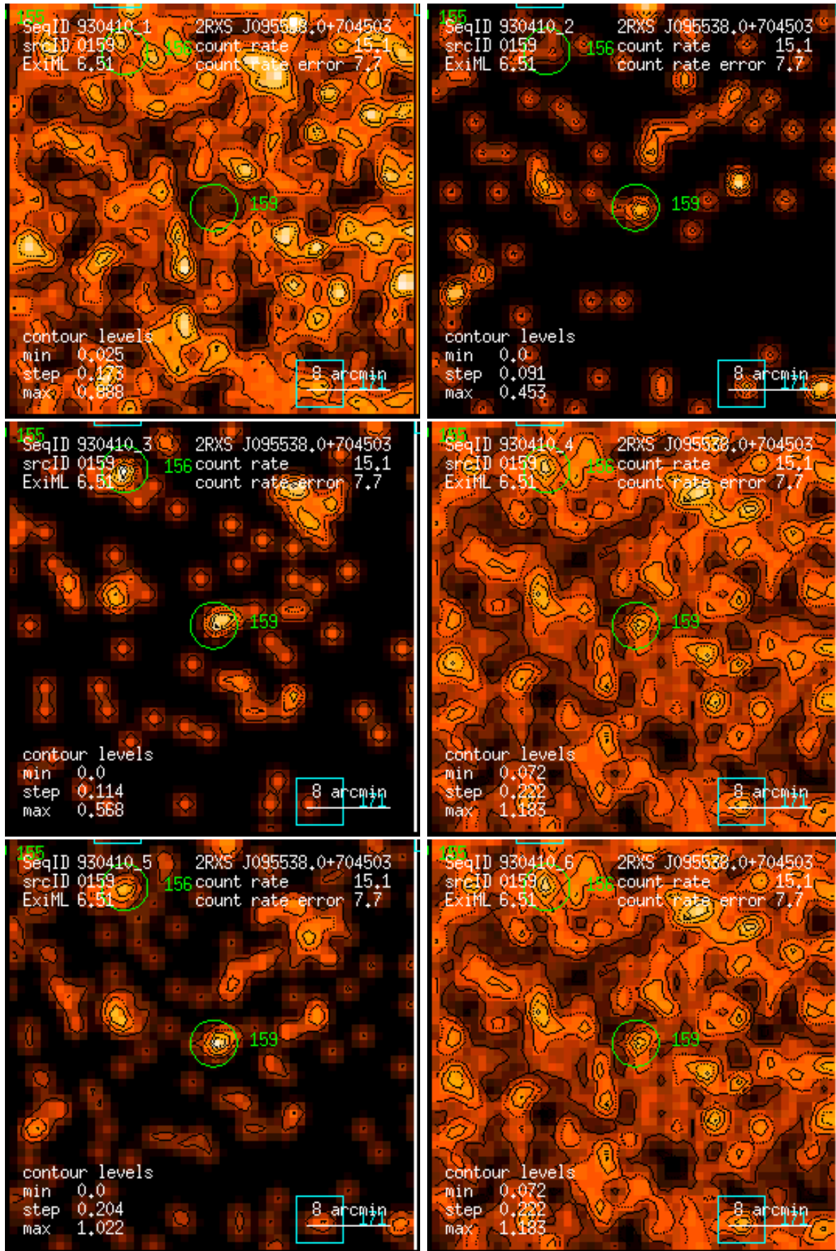
Figure 159: RASS 930410: detection 0159: band rate images, Gaussian filter: (1) PSPC channels 11 – 41, (2) 52 – 90, (3) 91 – 201, (4) 11 – 235, (5) 52 – 201, (6) 11 – 201. Broad band rates in counts/ks. Band rate contour levels in counts/ks/arcmin 2 .
