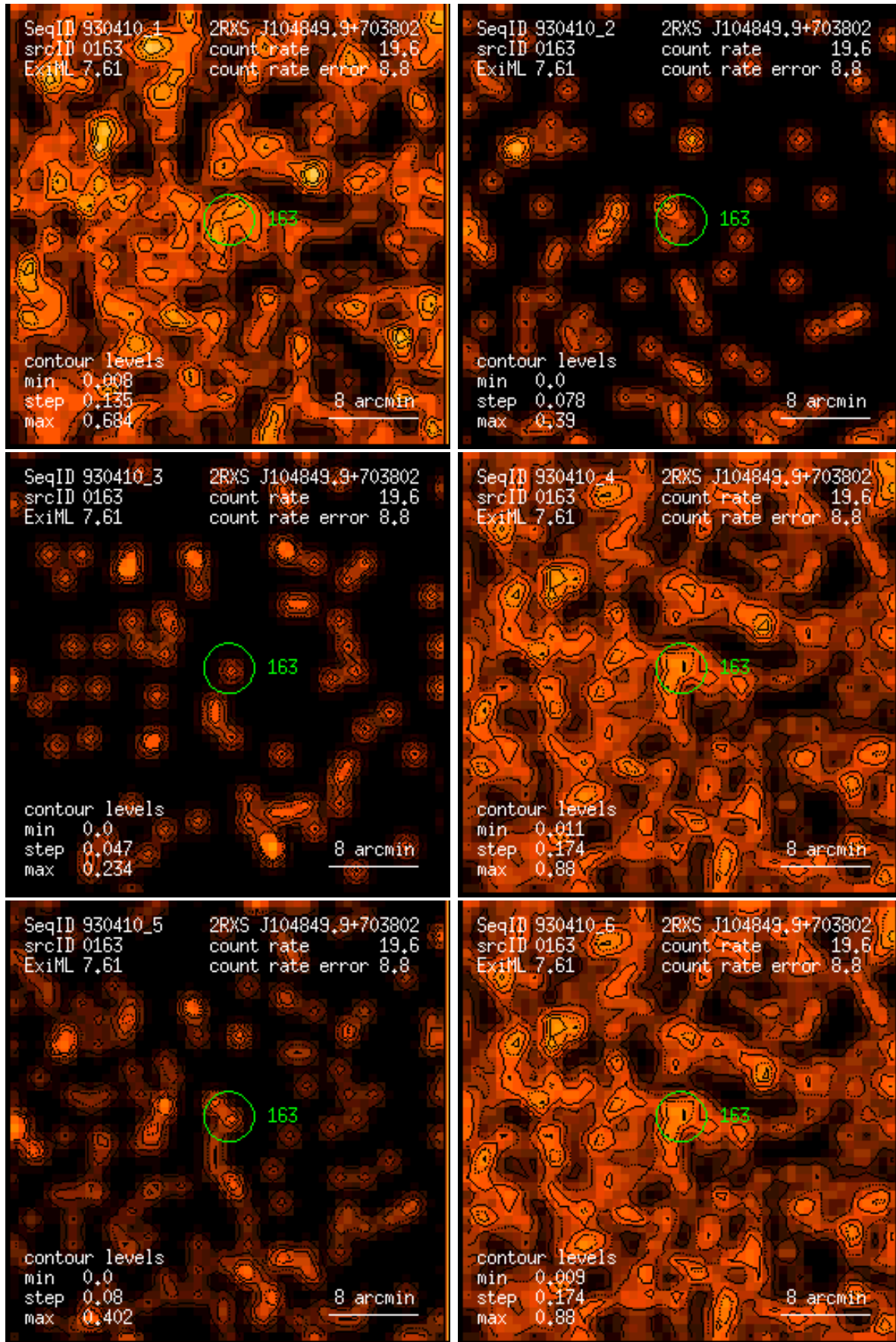
Figure 163: RASS 930410: detection 0163: band rate images, Gaussian filter: (1) PSPC channels 11 – 41, (2) 52 – 90, (3) 91 – 201, (4) 11 – 235, (5) 52 – 201, (6) 11 – 201. Broad band rates in counts/ks. Band rate contour levels in counts/ks/arcmin 2 .
