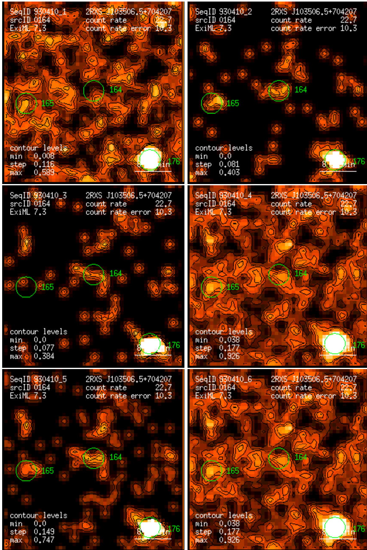
Figure 164: RASS 930410: detection 0164: band rate images, Gaussian filter: (1) PSPC channels 11 – 41, (2) 52 – 90, (3) 91 – 201, (4) 11 – 235, (5) 52 – 201, (6) 11 – 201. Broad band rates in counts/ks. Band rate contour levels in counts/ks/arcmin 2 .
