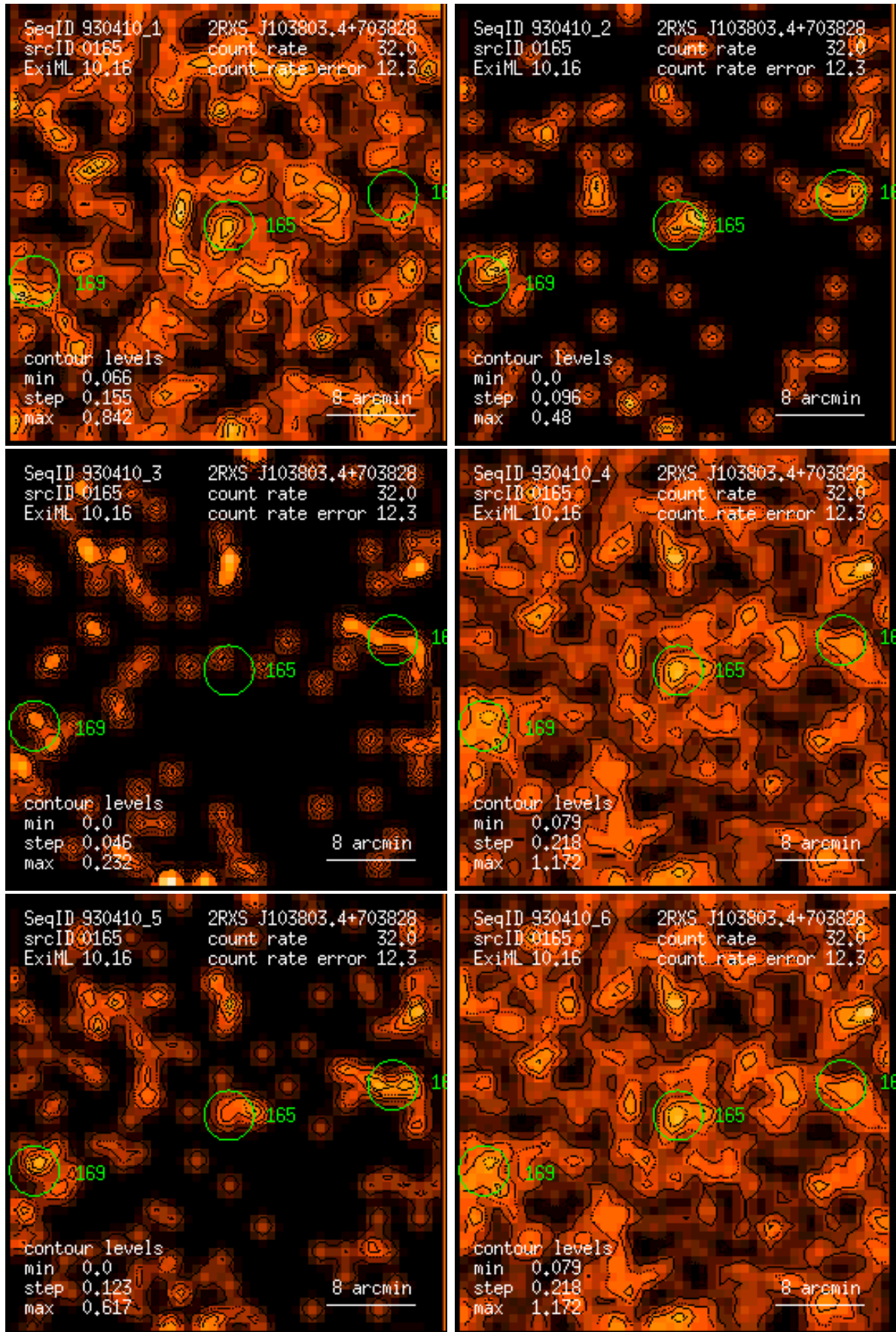
Figure 165: RASS 930410: detection 0165: band rate images, Gaussian filter: (1) PSPC channels 11 – 41, (2) 52 – 90, (3) 91 – 201, (4) 11 – 235, (5) 52 – 201, (6) 11 – 201. Broad band rates in counts/ks. Band rate contour levels in counts/ks/arcmin 2 .
