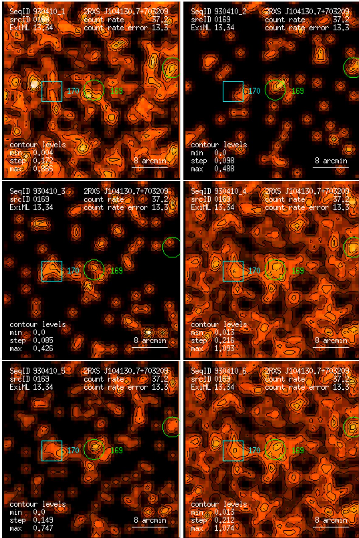
Figure 169: RASS 930410: detection 0169: band rate images, Gaussian filter: (1) PSPC channels 11 – 41, (2) 52 – 90, (3) 91 – 201, (4) 11 – 235, (5) 52 – 201, (6) 11 – 201. Broad band rates in counts/ks. Band rate contour levels in counts/ks/arcmin 2 .
