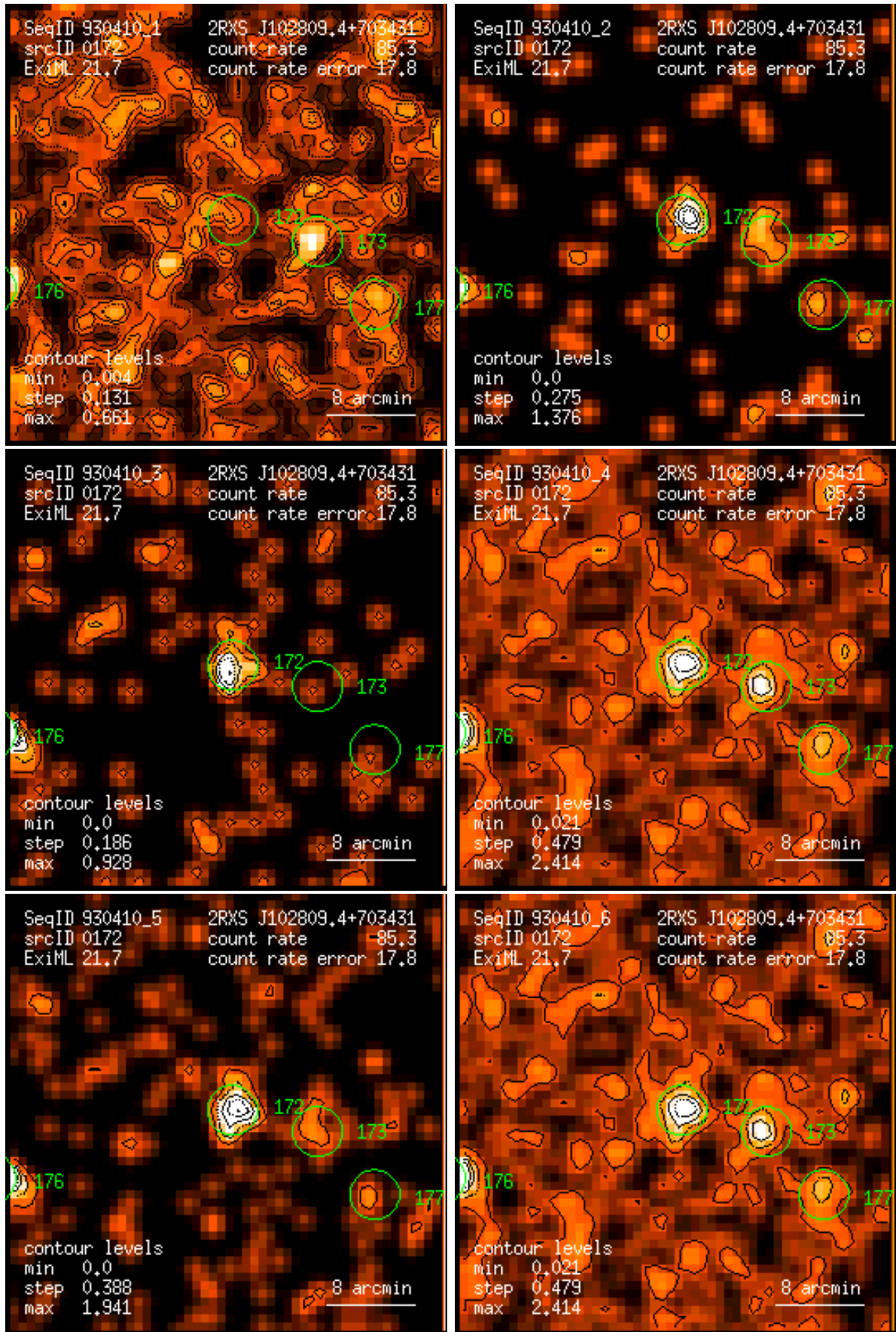
Figure 172: RASS 930410: detection 0172: band rate images, Gaussian filter: (1) PSPC channels 11 – 41, (2) 52 – 90, (3) 91 – 201, (4) 11 – 235, (5) 52 – 201, (6) 11 – 201. Broad band rates in counts/ks. Band rate contour levels in counts/ks/arcmin 2 .
