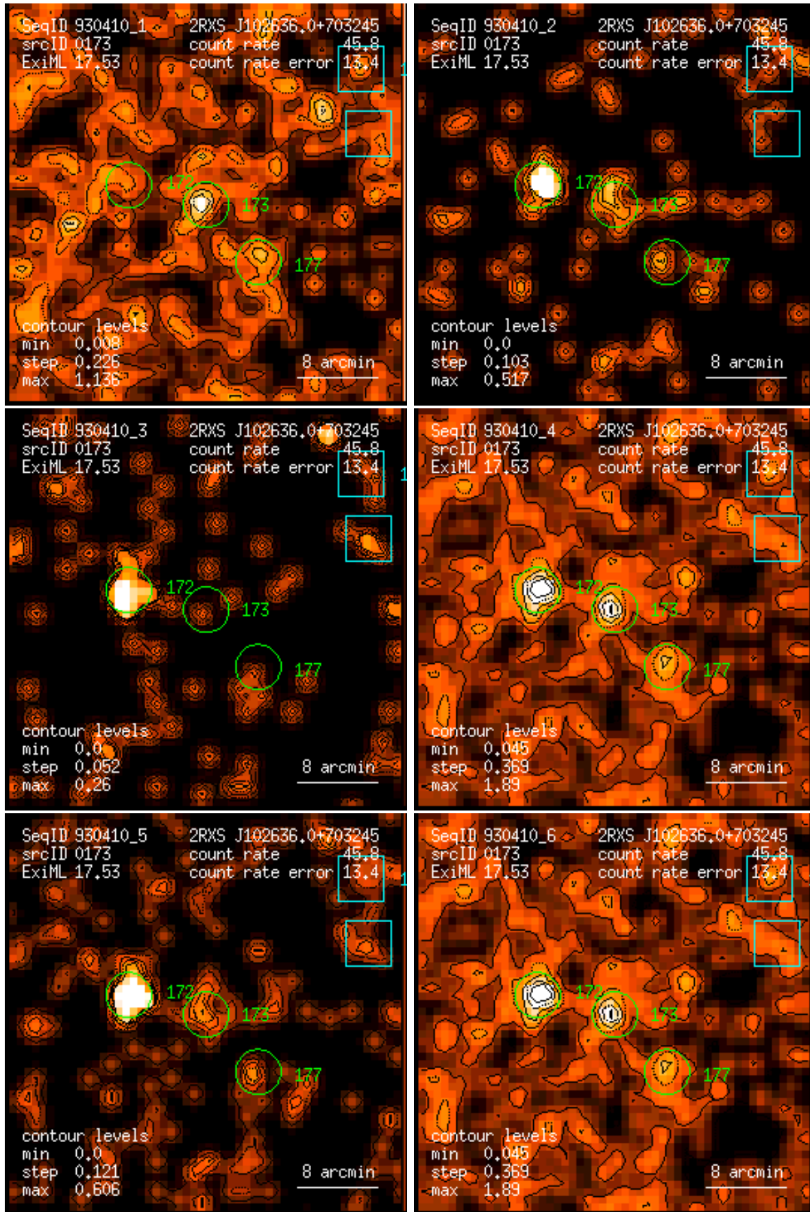
Figure 173: RASS 930410: detection 0173: band rate images, Gaussian filter: (1) PSPC channels 11 – 41, (2) 52 – 90, (3) 91 – 201, (4) 11 – 235, (5) 52 – 201, (6) 11 – 201. Broad band rates in counts/ks. Band rate contour levels in counts/ks/arcmin 2 .
