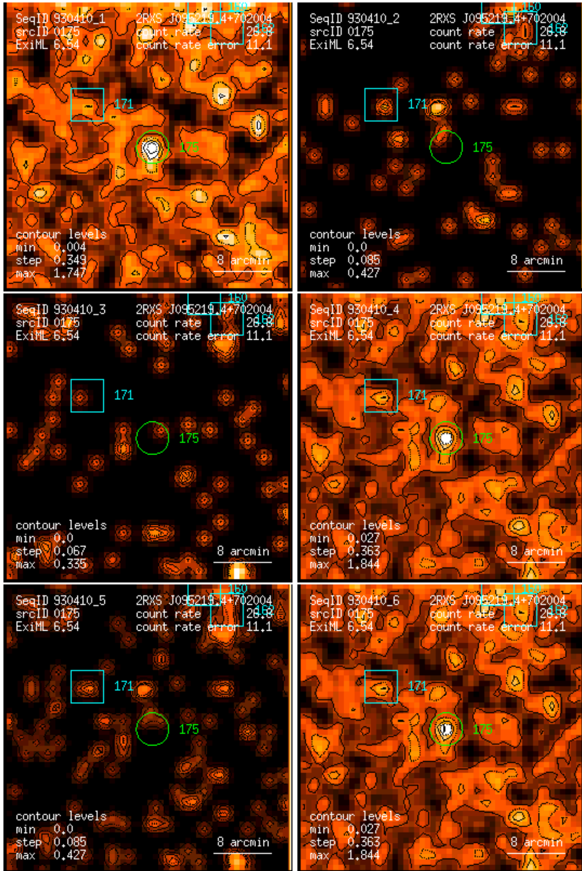
Figure 175: RASS 930410: detection 0175: band rate images, Gaussian filter: (1) PSPC channels 11 – 41, (2) 52 – 90, (3) 91 – 201, (4) 11 – 235, (5) 52 – 201, (6) 11 – 201. Broad band rates in counts/ks. Band rate contour levels in counts/ks/arcmin 2 .
