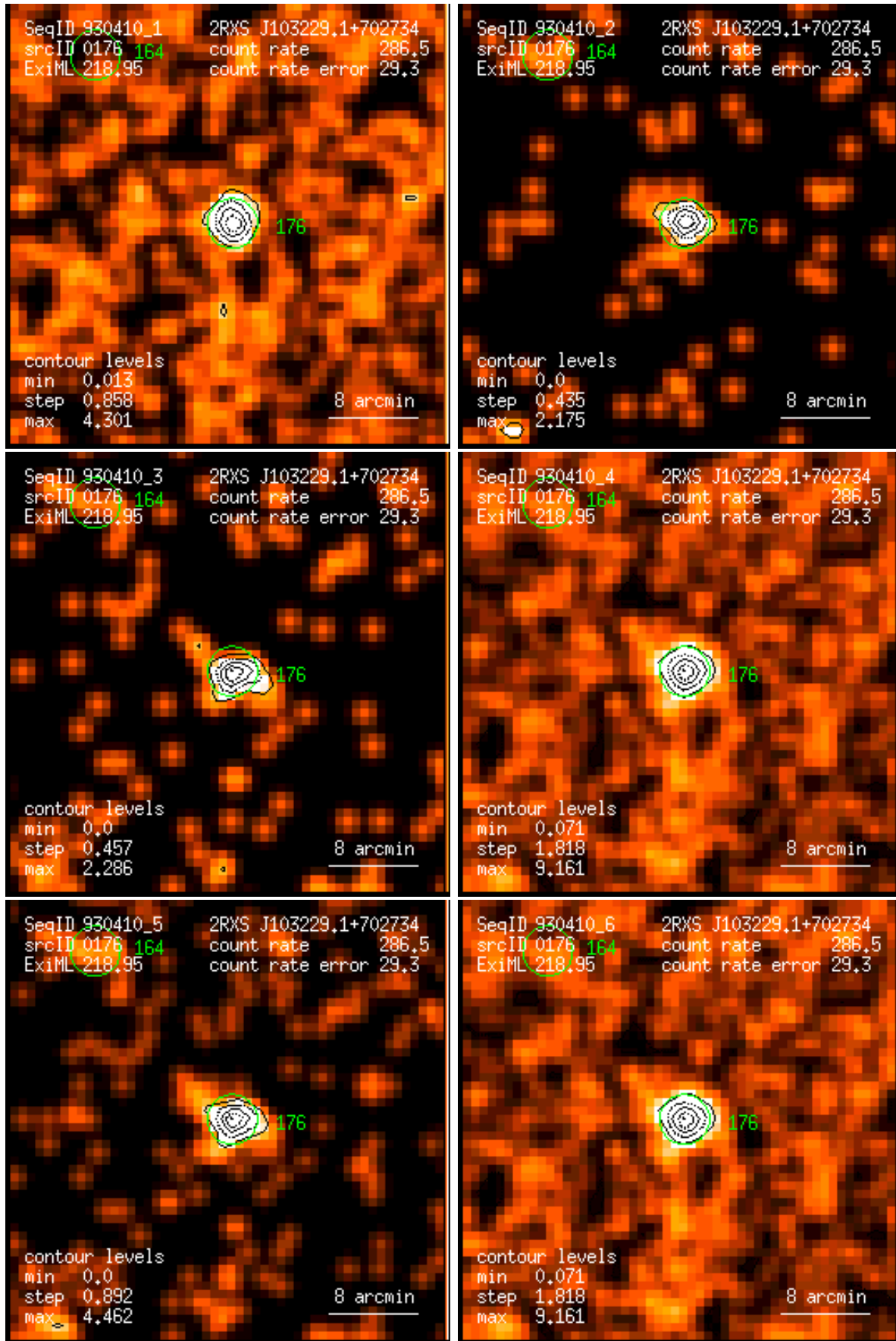
Figure 176: RASS 930410: detection 0176: band rate images, Gaussian filter: (1) PSPC channels 11 – 41, (2) 52 – 90, (3) 91 – 201, (4) 11 – 235, (5) 52 – 201, (6) 11 – 201. Broad band rates in counts/ks. Band rate contour levels in counts/ks/arcmin 2 .
