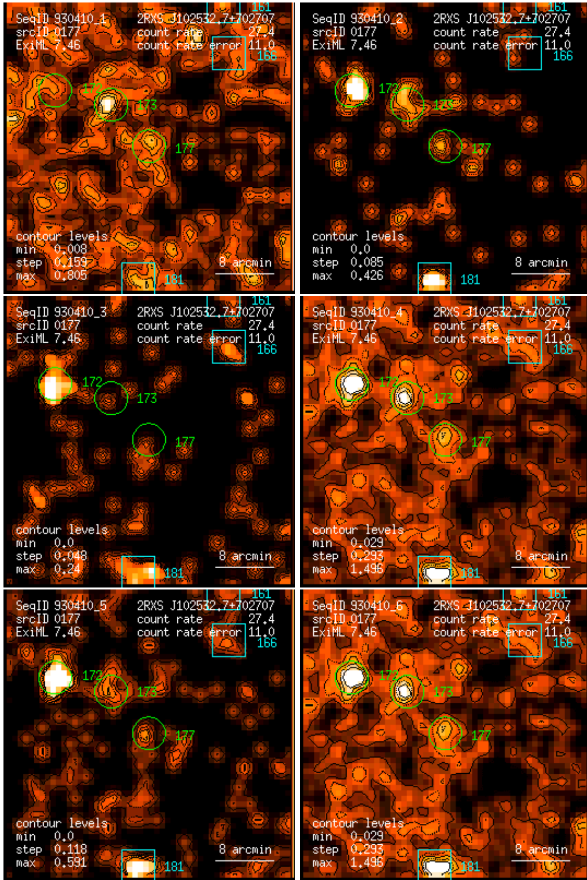
Figure 177: RASS 930410: detection 0177: band rate images, Gaussian filter: (1) PSPC channels 11 – 41, (2) 52 – 90, (3) 91 – 201, (4) 11 – 235, (5) 52 – 201, (6) 11 – 201. Broad band rates in counts/ks. Band rate contour levels in counts/ks/arcmin 2 .
