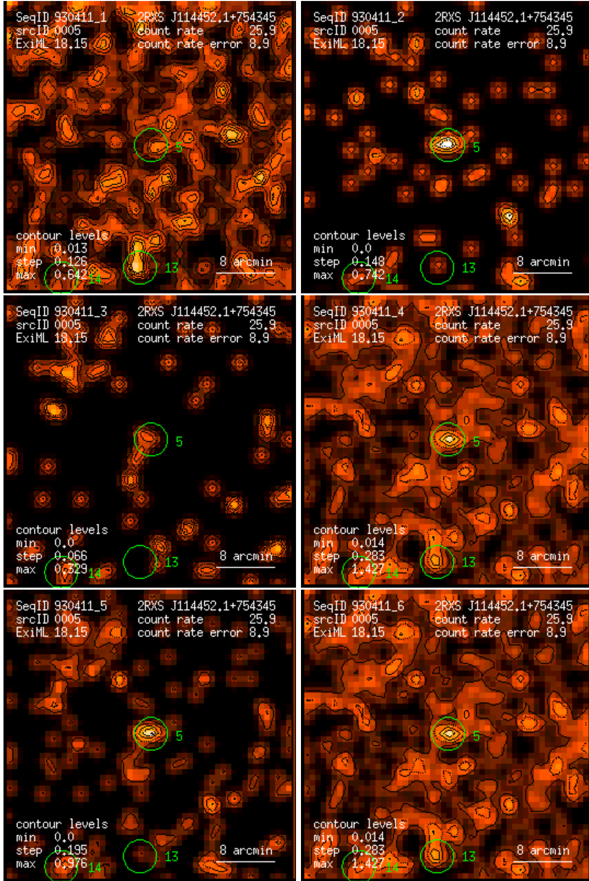
Figure 5: RASS 930411: detection 0005: band rate images, Gaussian filter: (1) PSPC channels 11 – 41, (2) 52 – 90, (3) 91 – 201, (4) 11 – 235, (5) 52 – 201, (6) 11 – 201. Broad band rates in counts/ks. Band rate contour levels in counts/ks/arcmin 2 .
