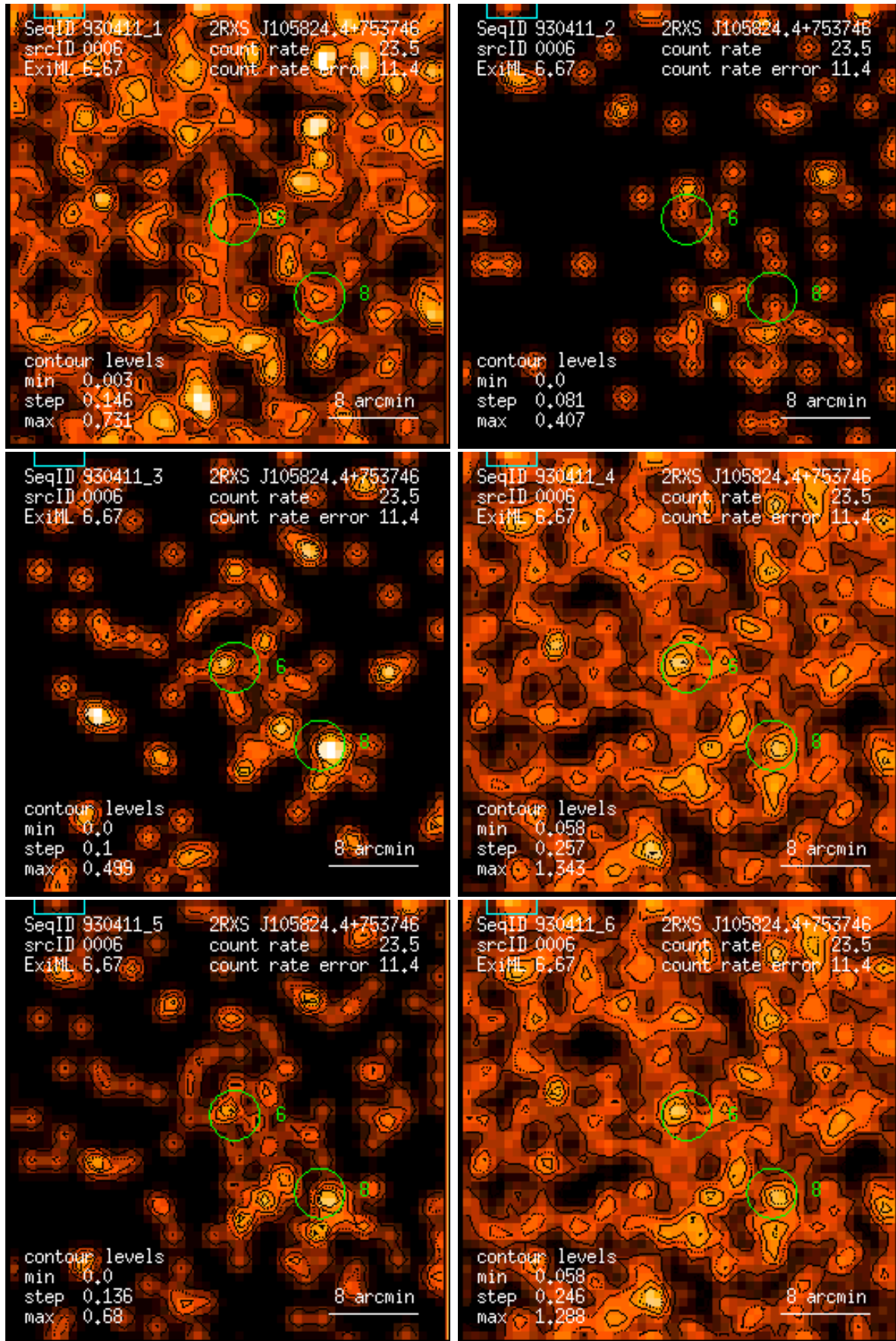
Figure 6: RASS 930411: detection 0006: band rate images, Gaussian filter: (1) PSPC channels 11 – 41, (2) 52 – 90, (3) 91 – 201, (4) 11 – 235, (5) 52 – 201, (6) 11 – 201. Broad band rates in counts/ks. Band rate contour levels in counts/ks/arcmin 2 .
